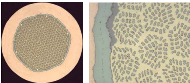
Figure 13: Bronze processed Nb 3 Sn strands with controlled bridging of filaments and low hysteresis losses.
