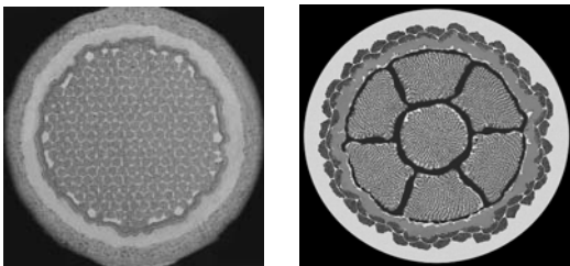
Figure 10: Strengthened by nanostructured CuNb alloy \text{Nb}_3\text{Sn} strands. Left: bronze processed strand with Cu-Nb layer replacing outer part of stabilizing Cu. Right: internal tin strand with Cu-Nb rods replacing the inner part of stabilizing Cu.
