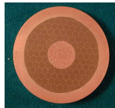
Figure 3: The Nb-Ti strand for ITER PF1&6 coils. Strand diameter: 0.73 mm, Cu/nonCu ratio: 1.6, filament diameter: 6.8 \mu\text{m} .
