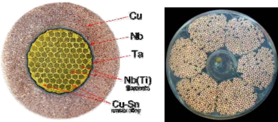
Figure 9: Left: cross section of stabilized bronze processed strand for ITER TFCI; diameter=0.81 mm, J_c @ 12T > 550 \text{A}/\text{mm}^2 , hysteresis losses ( \pm 3\text{T} ) < 200 \text{mJ}/\text{cm}^3 , RRR > 100 , Cu/(non Cu) = 1.5. Right: cross section of the cable in conduit conductor for TFCI.
