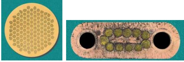
Figure 8: Left: Cross section of the Non stabilized bronze processed strand 1.5 mm in diameter; number of filaments: 14641; filaments diameter: 5 \mu\text{m} ; J_c @ 8 T: 510 \text{A}/\text{mm}^2 ; average I_c : 900 A. Right: cross section of conductor for T-15; critical current @ 8 T is \sim 11.5 kA, i.e., \sim 110\% of single strands current ability ( 11 \times 900 A).
