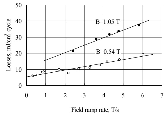
Figure 6: Hysteresis losses of the Nb-Ti trapezoidal cross section strand in different field ramp rates.
