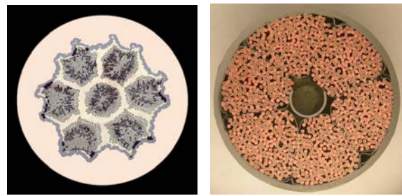
Figure 11: Cross sections of the internal tin \text{Nb}_3\text{Sn} strand, with J_c=830-950 \text{A}/\text{mm}^2 , Non-Cu hysteresis losses ( \pm 3\text{T} ; 4.2 K)=850-980 \text{kJ}/\text{m}^3 (left) and TF Conductor SULTAN sample, which met new ITER Specification Option 1 (right).
