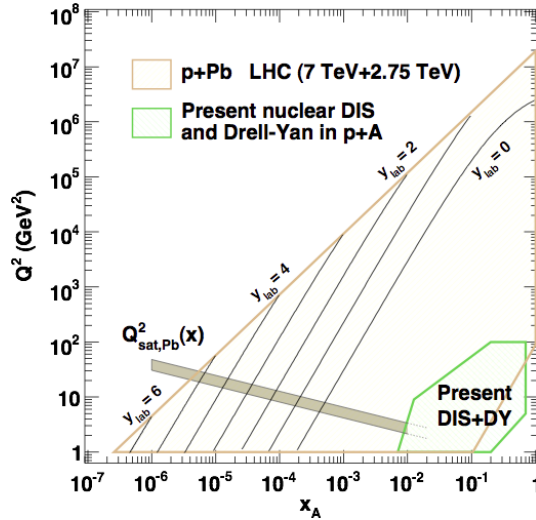
Figure 1. Kinematical coverage of the LHC proton-lead run compared with the one from earlier DIS and Drell-Yan (DY) experiments.
