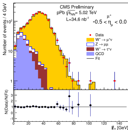
Figure 3. Missing transverse energy distribution for W^+ \rightarrow \mu^+ \nu in pPb collisions at \sqrt{s_{NN}} = 5.02 TeV within the -0.5 < \eta_{\text{lab}} < 0.0 range.
