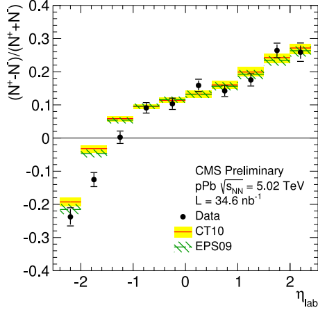
Figure 5. Charge asymmetry in W boson decays in pPb collisions at \sqrt{s_{NN}} = 5.02 TeV as a function of \eta_{lab}^l .
