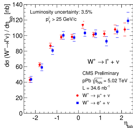
Figure 4. Production cross section for W^+ \rightarrow \ell^+ \nu in pPb collisions at \sqrt{s_{NN}} = 5.02 TeV as a function of \eta_{\text{lab}}^\ell .
