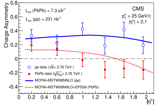
Figure 2. Muon charge asymmetry in W boson decays as a function of muon pseudo-rapidity for pp and PbPb collisions at \sqrt{s_{NN}} = 2.76 \text{ TeV} .
