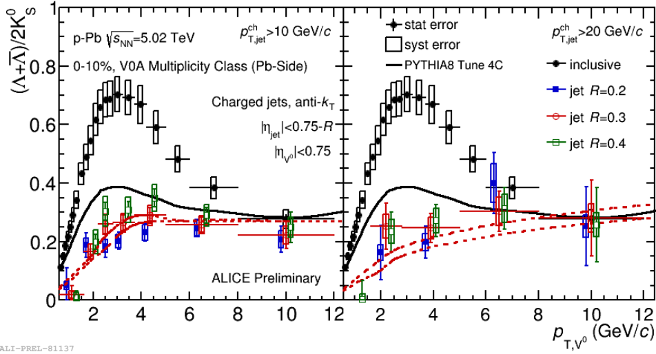
Figure 2. \Lambda/K_S^0 ratio in charged jets with R = 0.2, 0.3, 0.4 in p–Pb collisions at \sqrt{s_{NN}} = 5.02 TeV for p_T^{\text{jet, ch}} > 10 GeV/c (left) and p_T^{\text{jet, ch}} > 20 GeV/c (right), compared with the inclusive ratio and simulation results. Black solid line indicates the inclusive ratio from PYTHIA 8. Red dashed lines denote the spread of ratios in PYTHIA jets for all used values of R .
