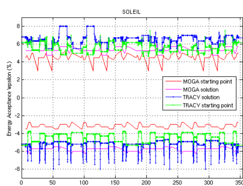
MA comparison between MOGA and TRACY solutions for the ideal storage ring model
