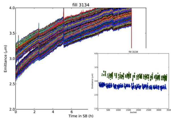
Figure 5: Bunch by bunch luminosity convoluted emittance versus time during physics fill 3134 of the LHC in 2012.
