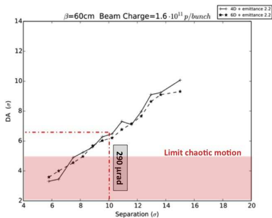
Figure 4: Dynamic Aperture as a function of the beam-beam separation at first long range encounter for a beam with 1.6 \cdot 10^{11} proton per bunch. The red region identifies the chaotic motion region.
