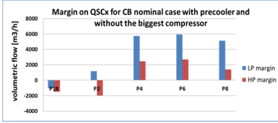
Figure 8: Helium flow margins for compressor stations.
