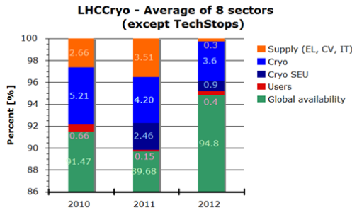
Figure 4: Cryogenic availability – Run1 summary.
