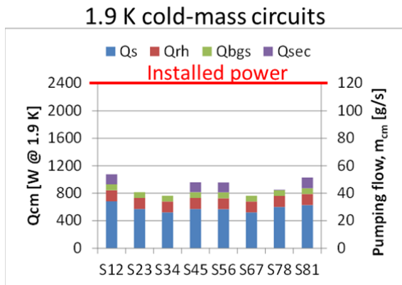
Figure 15: cold mass heat load and available cooling power.
