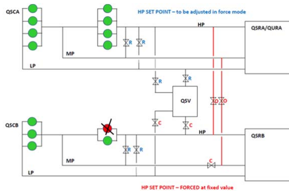
Figure 7: Configuration of linked compressor stations.
