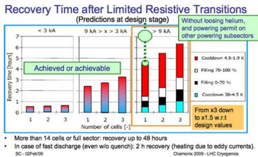
Figure 12: Recovery after quenches
