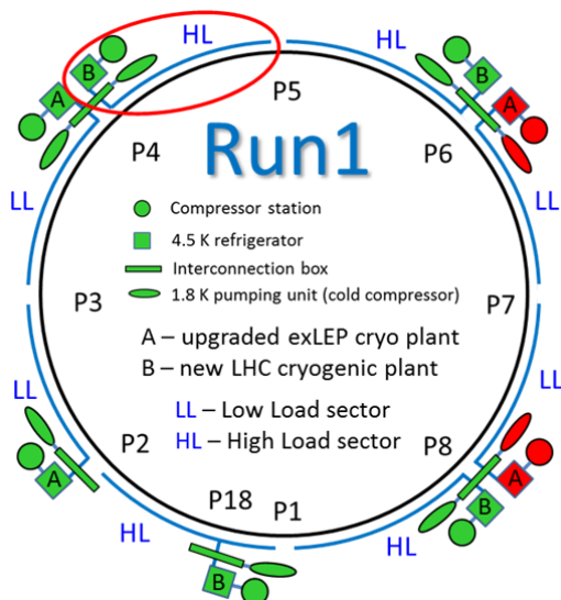
Figure 1: LHC cryogenic infrastructure.
