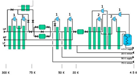
Figure 9: Air Liquide QSRB – turbines criticality.
