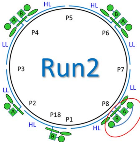
Figure 6: Baseline for LHC Run2 operation scenario.
