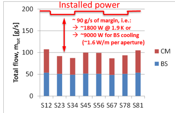
Figure 15: Global cooling margin
