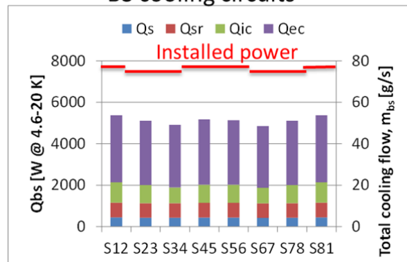
Figure 14: BS heat load and available cooling power.
