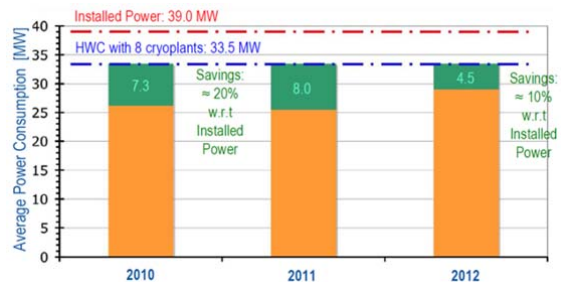
Figure 2: Power consumption and savings during Run1.
