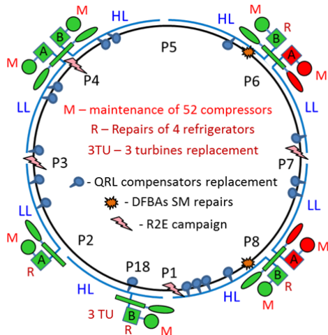
Figure 5: Main activities on cryogenic system during LS1.
