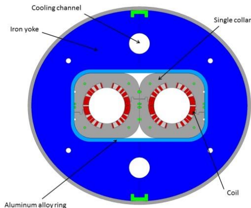
Figure 9: Cross-section of the recombination dipole D2.
