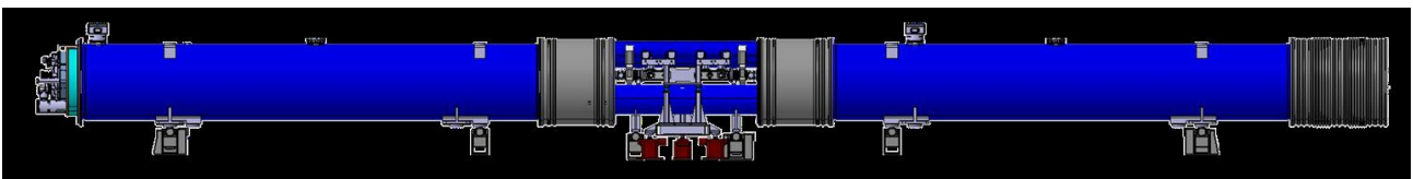
Figure 2: The 11 T unit, composed of two 5.5-m-long magnets with a room temperature collimator
