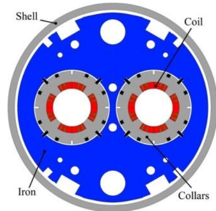
Figure 10: Cross-section of the quadrupole Q4.
