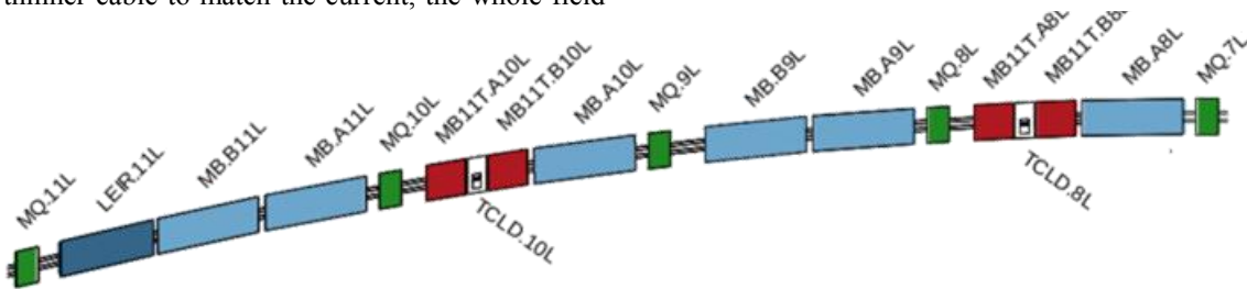
Figure 1: Replacement of an 8.3 T LHC dipole with 11 T dipole plus collimator
