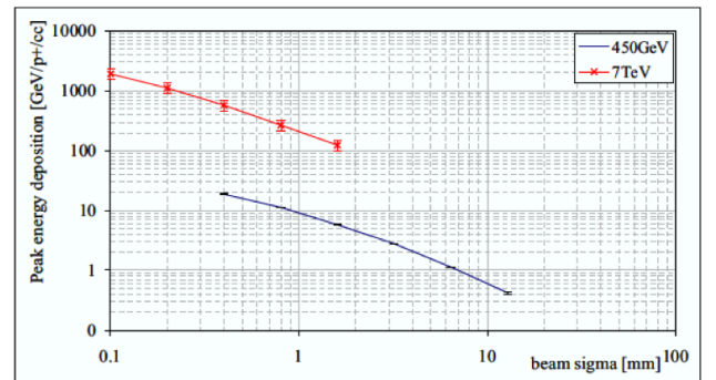
Figure 1: Peak energy deposition in Cu for 450 GeV and 7 TeV as a function of the spot size. Round beams were assumed in the FLUKA simulations.
