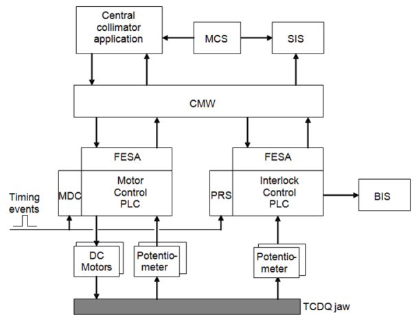
Figure 8: Upgraded TCDQ electronics with position control and readout in separate PLCs [3].
