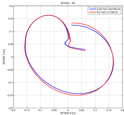
Figure 10: Beam dilution on the dump screen after LS1. Courtesy M. Fraser.
