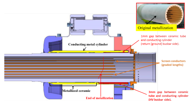
Figure 1: Improved MKI beam screen with 24 graded length conductors and a conducting metal cylinder with a vacuum gap of between 1 to 3 mm to the ceramic tube.
