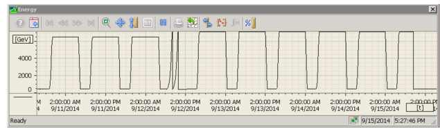
Figure 12: Cycling of the MKD generators up to 7 TeV without self triggers.
