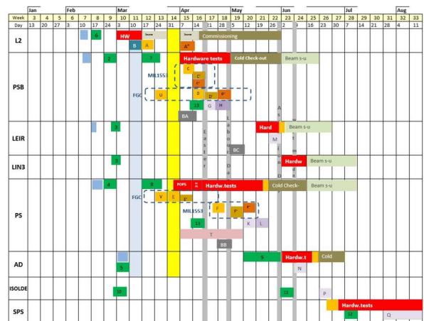
Figure 3: Planning of controls dry runs per machine.
