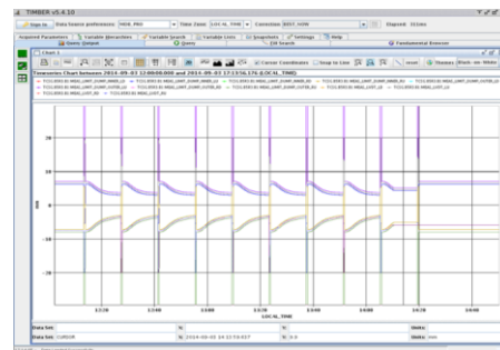
TCSG.B5R3.B1 jaw positions and threshold of as logged in timber during reliability test.
