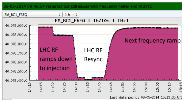
Fig 2: Signal from Alice Frequency meter
