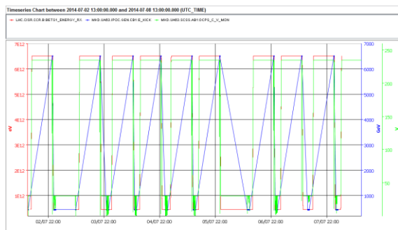
Fig 4: LBDS reliability run
