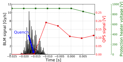
Figure 4: BLM signals and QPS signals recorded during the fast orbit-bump quench test in MQ.12L6.
