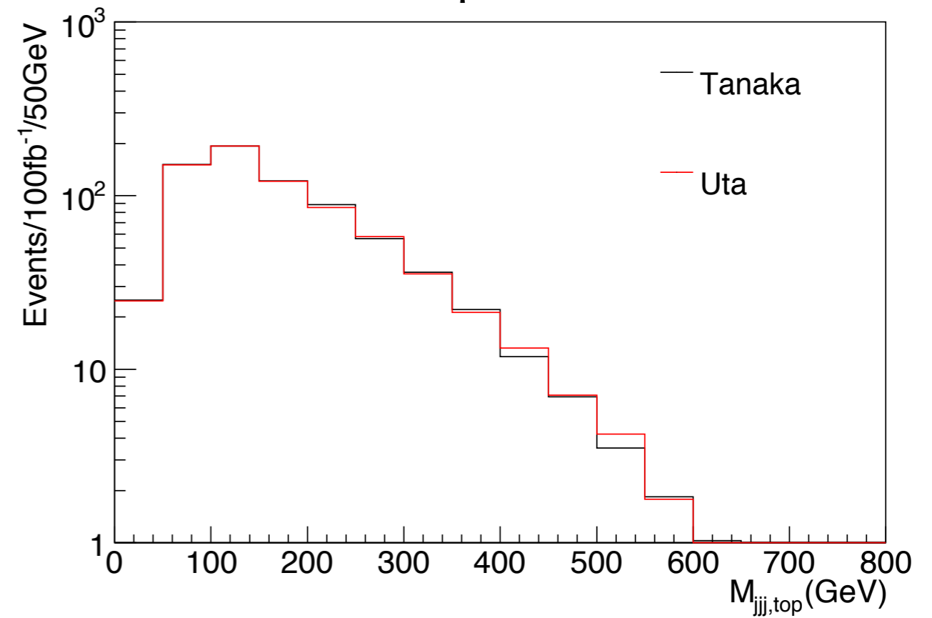
Top mass
