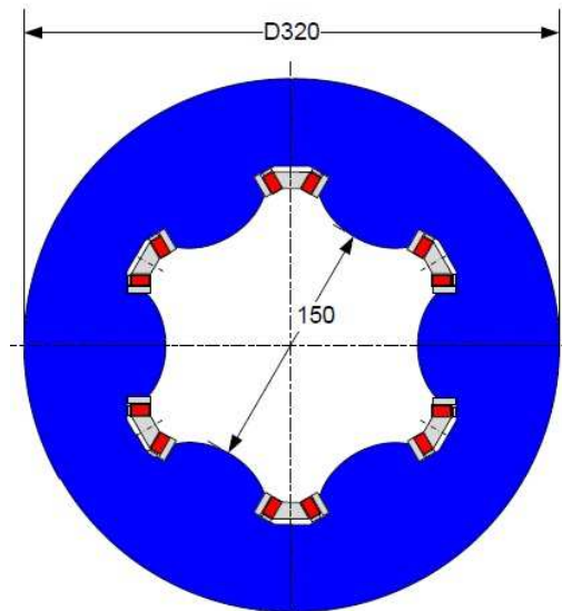
Fig. 1: Sketch of the cross-section (skew case)
