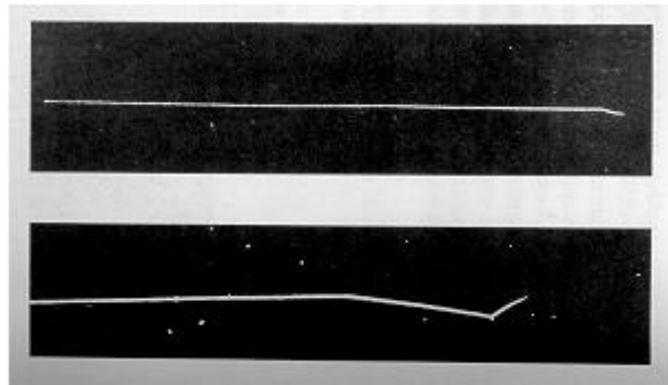
Early Alpha-Ray picture, Wilson 1912
