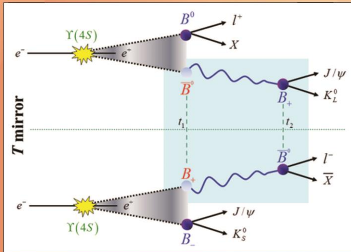
COLLOQUIUM: TIME-REVERSAL VIOLATION WITH QUANTUM-ENTANGLED B MESONS
