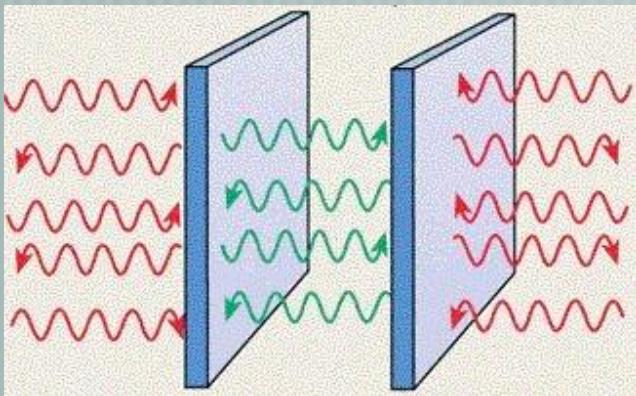
Casimir effect (force on two uncharged metal plates)
