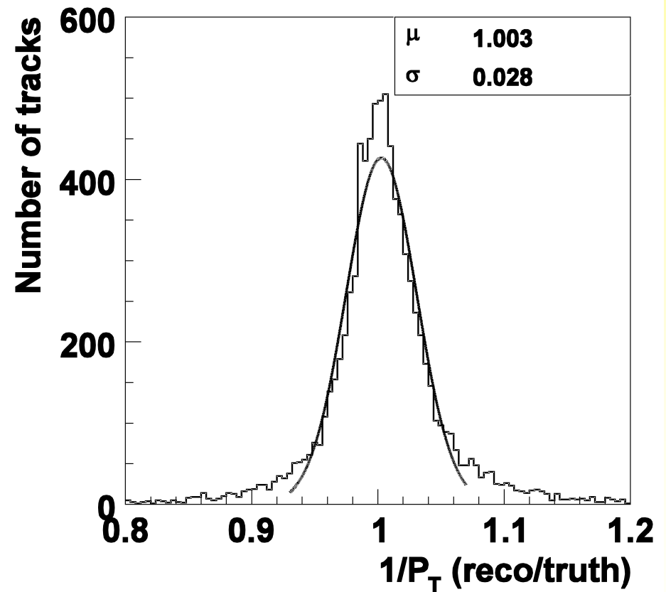
Refit with Global- \chi^2 Fitter
