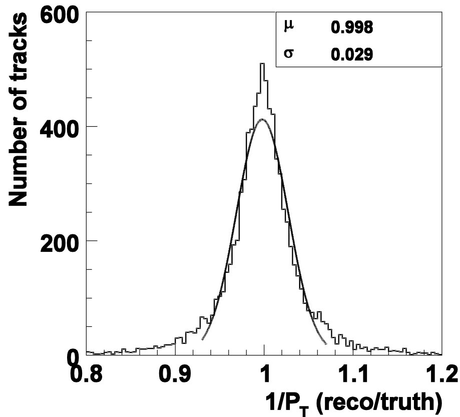
Muon reconstruction
