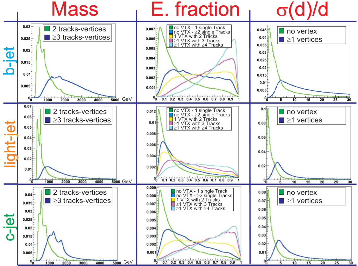
Figure 7. The PDFs for the mass, the energy fraction and the flight length significance are shown, separately for the three different jet-flavours and split according to the decay chain topology found by JetFitter .
