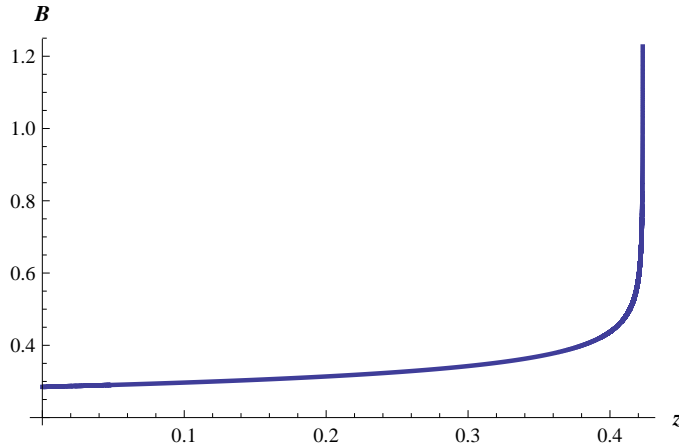
Figure 3: The function B(z) for integration constant t_1 = 0.1 .
