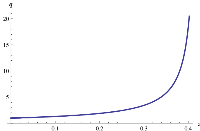
Figure 2: The function q(z) for integration constant t_1 = 0.1 .
