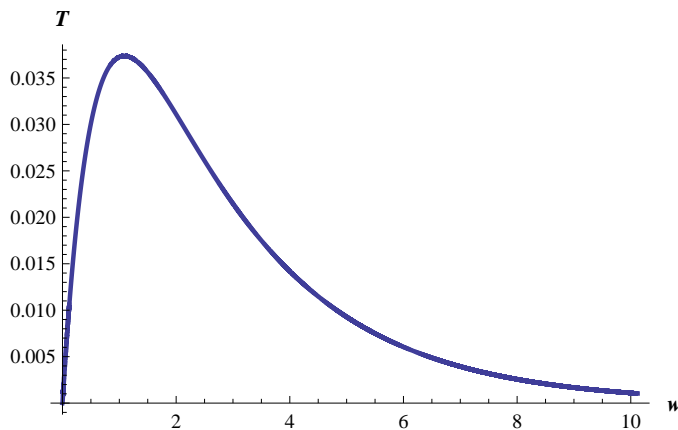
Figure 1: The function T(w) for integration constant t_1 = 0.1 .
