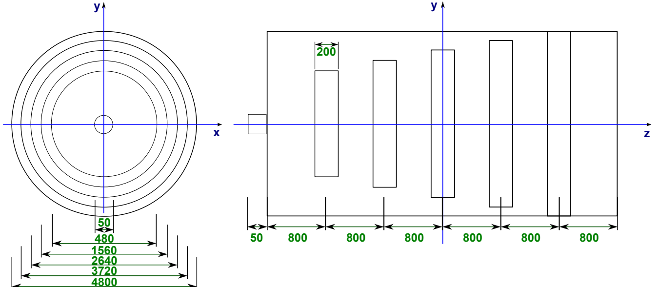
Figure 1: Layout of the experimental setup [size in millimeter]
