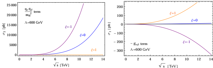
Figure : Total parton-level cross sections versus energy, for \Lambda = 600 GeV and various \xi .
