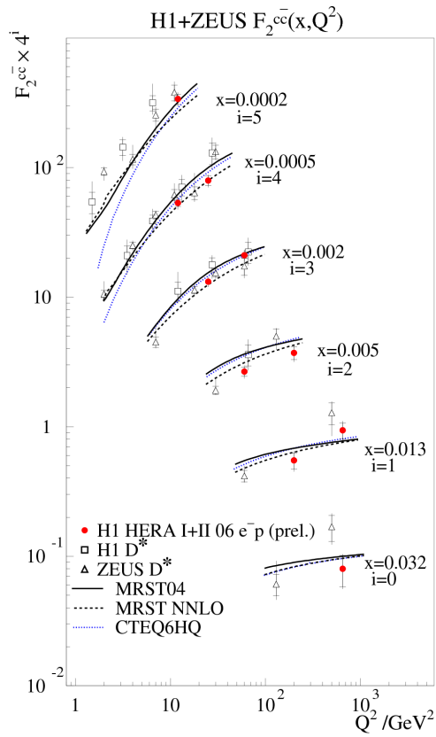
Figure 16. F_2^{c\bar{c}} as a function of Q^2 for different x ranges. Also shown are measurements from the H1 and ZEUS collaborations using D^* mesons to identify the charm quarks. The inner error bars show the statistical uncertainty, the outer error bars represent the statistical and systematic uncertainties added in quadrature.
