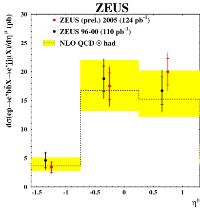
Figure 8. b -quark production cross-section in di-jet photoproduction as a function of the pseudorapidity of the muon. The measurement is compared to an earlier ZEUS publication [ 9] and the NLO QCD prediction. The uncertainty on the prediction is indicated by the band.
