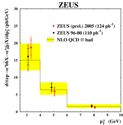
Figure 7. b -quark production cross-section in di-jet photoproduction as a function of the transverse momentum of the muon. The measurement is compared to an earlier ZEUS publication [ 9] and the NLO QCD prediction. The uncertainty on the prediction is indicated by the band.
