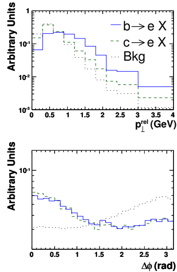
Figure 9. Variables used to separate semileptonic heavy quark decays from background. The solid line shows the distribution for electrons from semileptonic b -quark decays, the dashed line for c -quark decays and the dotted line the background (Bkg).
