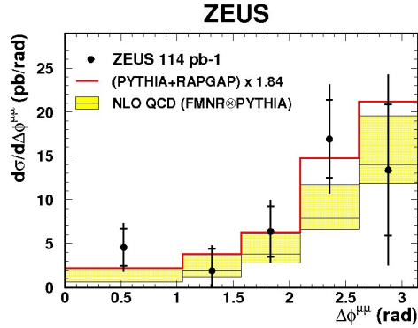
Figure 12. The dimuon cross-section as a function of the azimuthal angle between the muons in dijet events. The data (points) are compared to the NLO QCD prediction calculated using the FMNRxPYTHIA interface as well as to the RAPGAP prediction scaled by a factor of 1.84. The inner error bar shows the statistical uncertainty and the outer error bar shows the statistical and systematic uncertainties added in quadrature.
