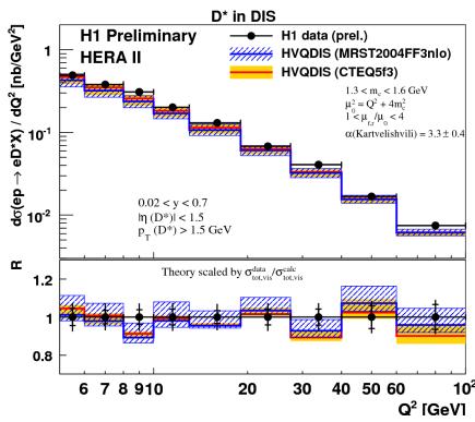
Figure 3. D^* production cross-section as a function of Q^2 . The data (points) are compared to NLO QCD predictions with two different PDFs. The lower plot shows the NLO QCD prediction scaled by the ratio of the data to NLO QCD visible cross-sections. The range of variation of the quark mass and factorisation and renormalisation scales are indicated in the figure.
