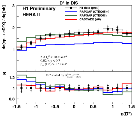
Figure 6. D^* production cross-section in DIS as a function of \eta(D^*) . The data are compared to the different Monte Carlo generators as indicated in the figure.
