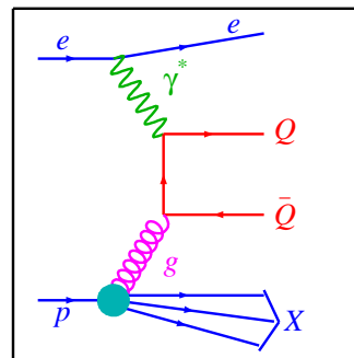
Figure 1. Feynman diagram of the boson gluon fusion process.
