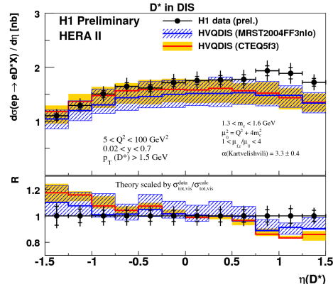
Figure 4. D^* production cross-section in DIS as a function of \eta(D^*) compared to NLO QCD predictions. For further details see the caption of Figure 3.
