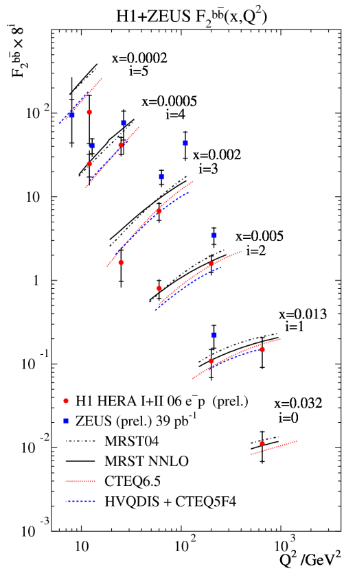
Figure 17. F_2^{b\bar{b}} as a function of Q^2 for different x ranges. Also shown is a preliminary measurement from the ZEUS collaboration using the data from 2004. The inner error bars show the statistical uncertainty, the outer error bars represent the statistical and systematic uncertainties added in quadrature.
