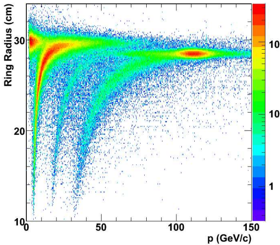
RICH Ring Radius vs. Momentum
