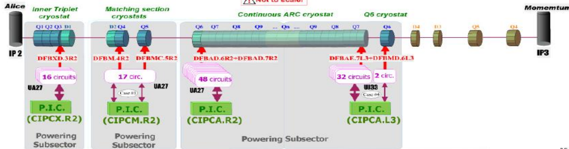
POWERING SUBSECTORS for the Sector between IP2 and IP3
