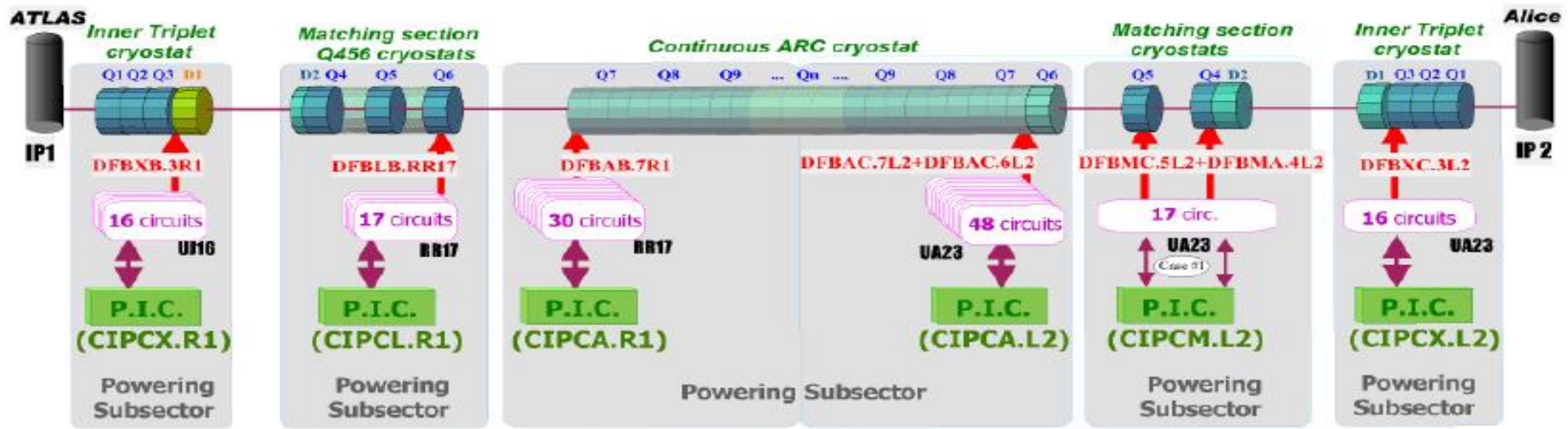
POWERING SUBSECTORS for the Sector between IP1 and IP2
