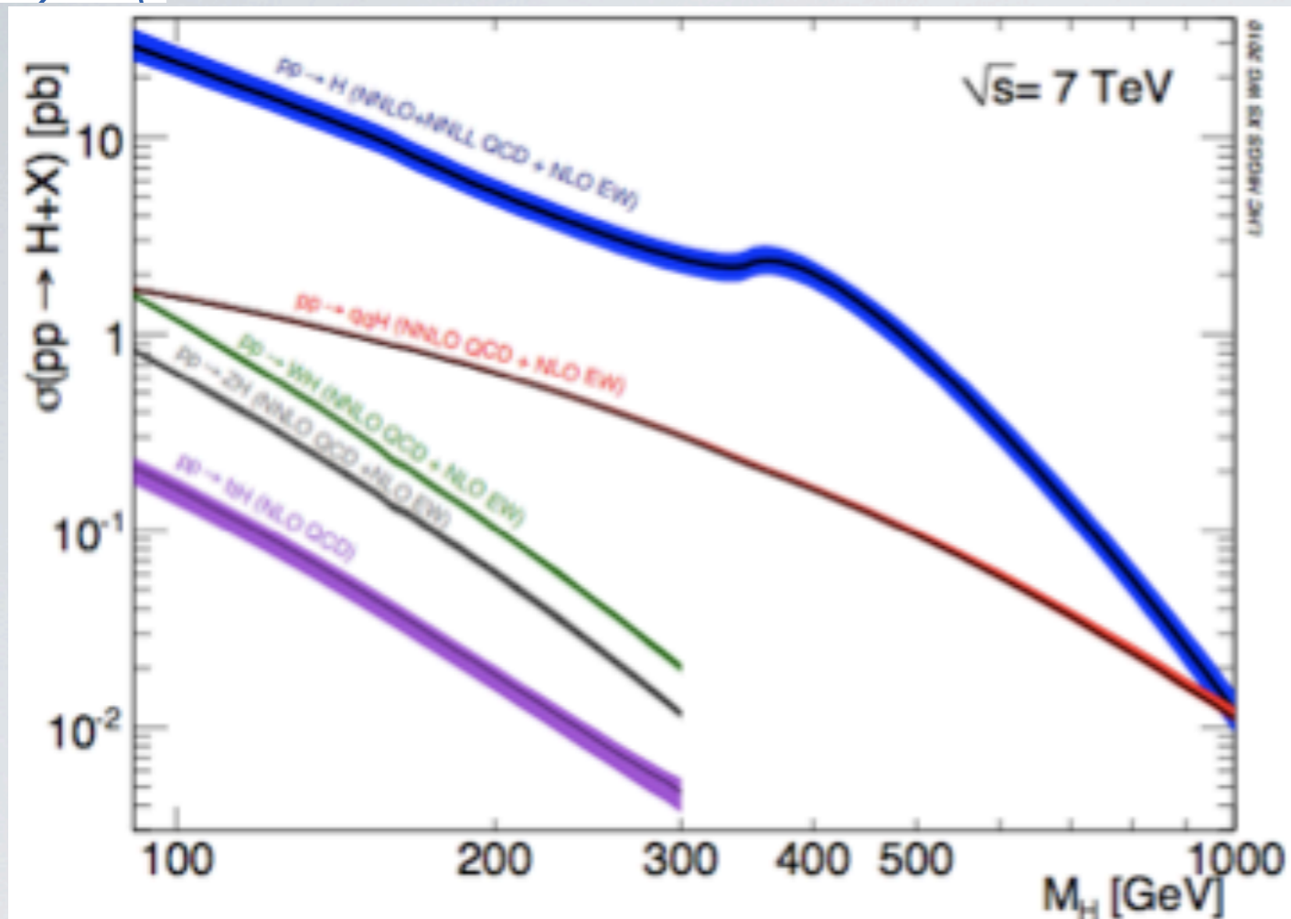
gluon-fusion
