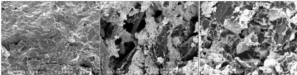
Figure 2. SEM images. From left to right: compact structure of high-density UC, open structure containing UC 2 grains and carbon fibers, open structure containing UC 2 grains and graphite residual clusters (black blocks).
