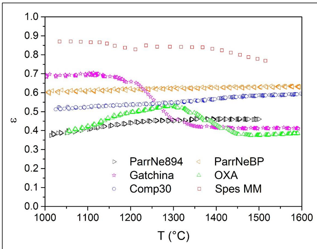
Figure 8. Thermal emissivity of different types of uranium carbide.
