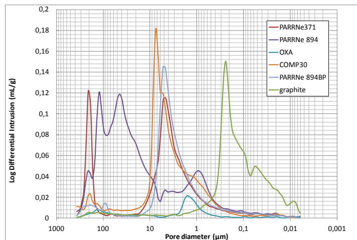
Figure 3. Pore size distribution of different samples using mercury porosimetry.
