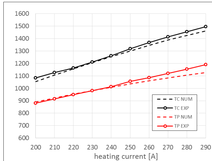
Figure 6. Experimental and numerical temperatures on center and periphery of a UC x disc.
