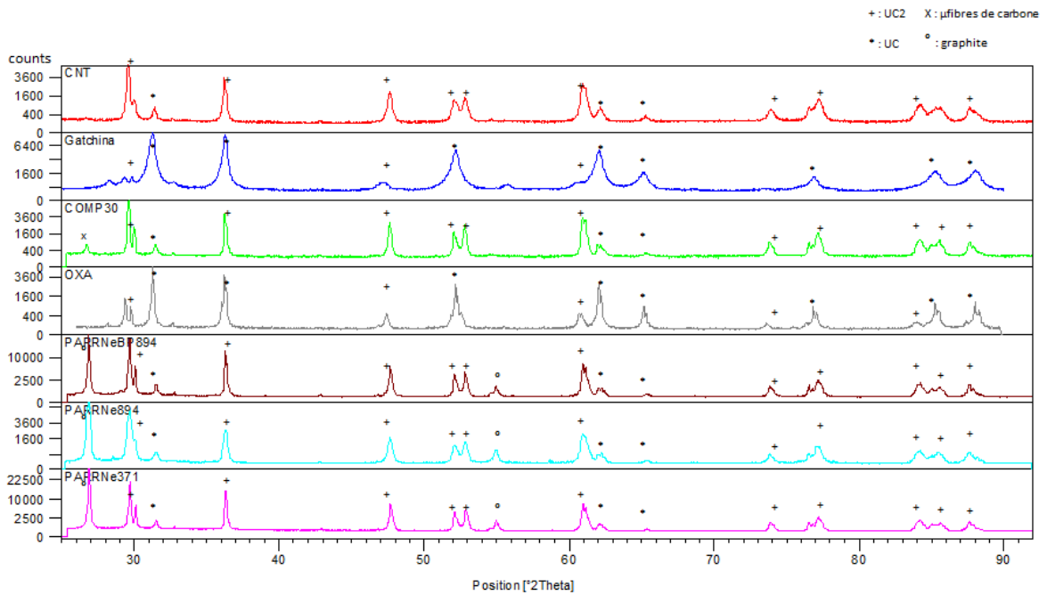
Figure 1. XRD patterns of different samples, highlighting the presence of UC, UC 2 , graphite and carbon microfibres.
