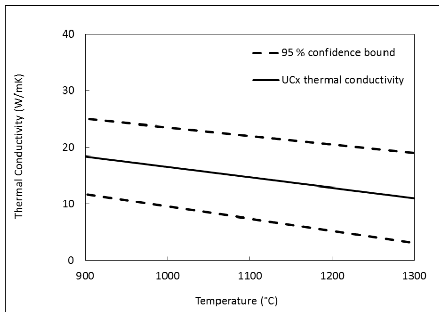
Figure 7. Thermal conductivity of UC x .
