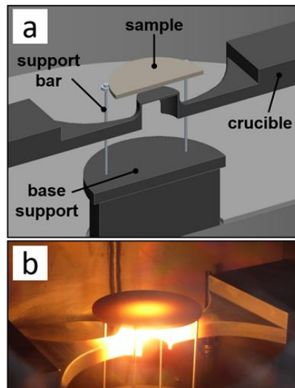
Figure 5: a) CAD view of the thermal conductivity estimation setup, b) sample heated by irradiation by the crucible, with the creation of a temperature gradient.
