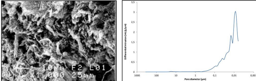
Figure 4: SEM picture of a UC_x synthesized with CNTs correlated to a spectrum obtained by Hg porosimetry. These data show the porous structure of CNTs and UC_2 (white color) growing on CNTs.
