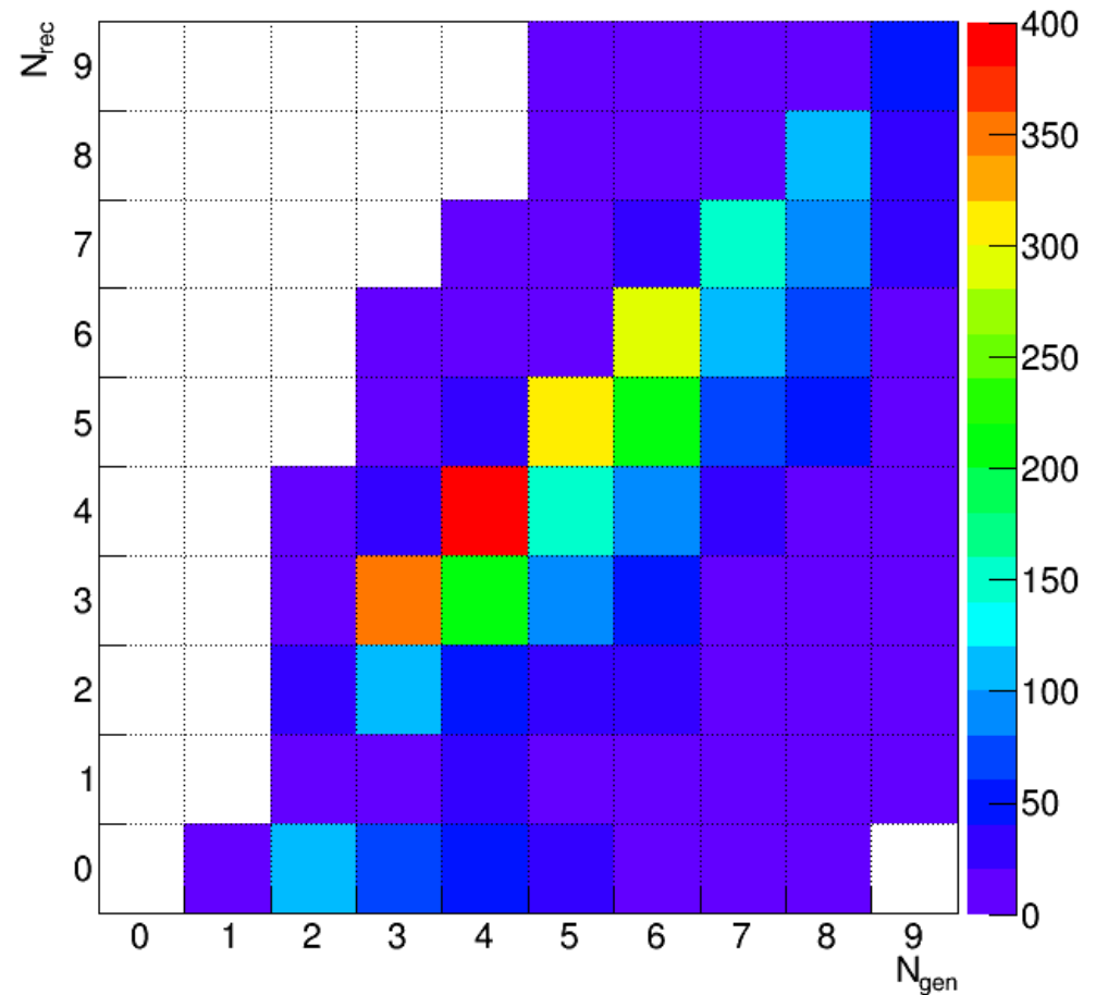
Btag > 0.3
