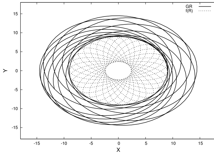
Fig. 1 Example of massive particle equatorial trajectories in a Kerr and axially-symmetric f(R) metric, obtained from the solution of the Hamilton-Jacoby equations (13). In both cases the BH spin is a = 0.5 , and for f(R) we employed \alpha = 10 and \beta = 5 for representative purposes. The test mass at the beginning has a pure tangential velocity component d\phi/dt = 0.03 and is placed at 9R_g
