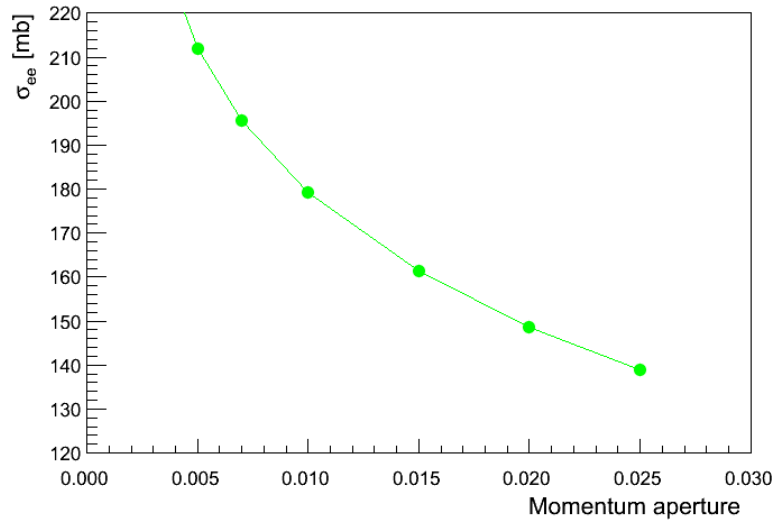
Figure 1: Evolution of the radiative Bhabha cross-section evaluated with BBRM as a function of the momentum aperture at a beam energy of 120 GeV.
