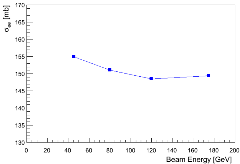
Figure 2: Dependence of the radiative Bhabha cross-section on the beam energy for a momentum acceptance of 2%.
