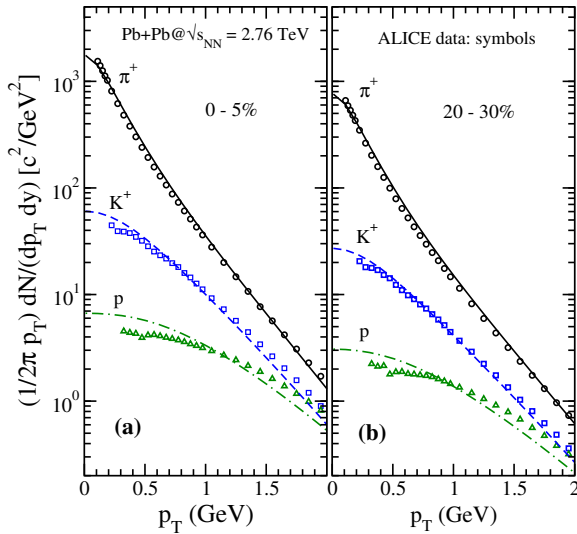
Figure 1. Transverse momentum distribution of \pi^+ , K^+ and p multiplicities in Pb+Pb collisions at \sqrt{s_{NN}} = 2.76 TeV in two centrality ranges, (a): 0–5% and (b): 20–30%. The symbols represent ALICE data [13] at mid-rapidity and the lines correspond to viscous blast-wave results.
