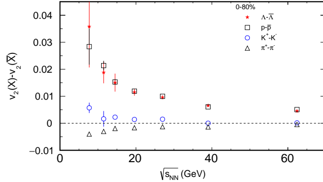
Figure 3. The difference in v_2 between particles ( X ) and their corresponding antiparticles ( \bar{X} ) as a function of beam energy for 0 – 80% central Au + Au collisions [10, 11].
