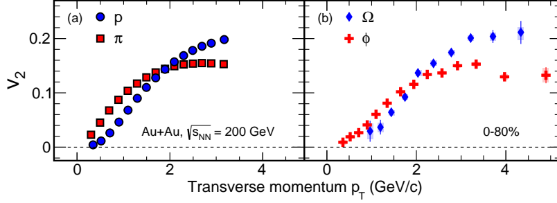
Figure 1. The v_2 as function of p_T for \pi ( \pi^+ + \pi^- ), p ( p + \bar{p} ) and \phi , \Omega ( \Omega^- + \bar{\Omega}^+ ) in Au+Au collisions at \sqrt{s_{NN}} = 200 GeV for 0-80% centrality [6].
