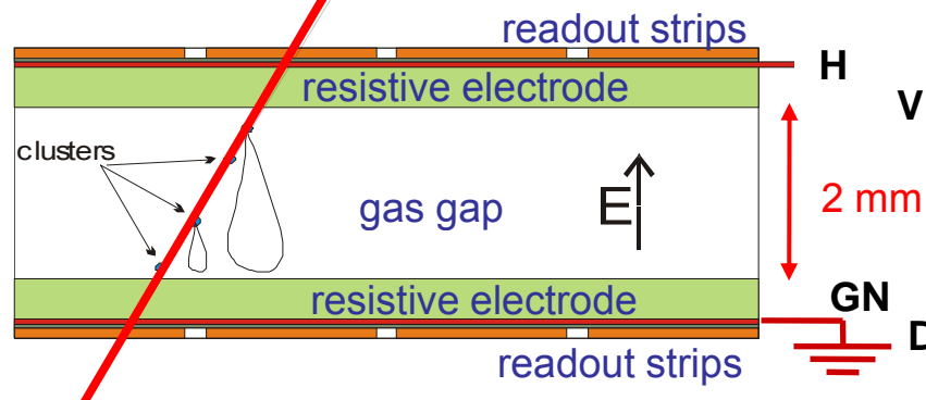
Resistive Platechamber
