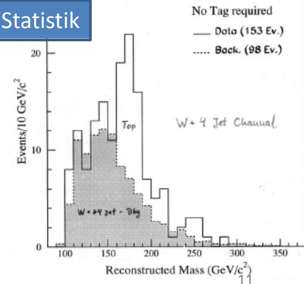
TOP-QUARK-SIGNAL
