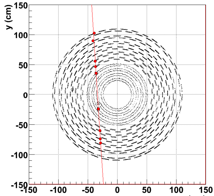
Run 50908 Event 96, y vs x
