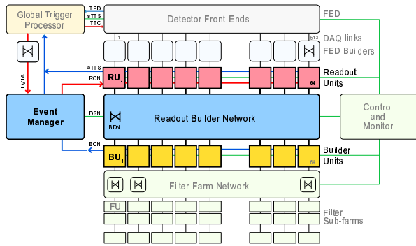
Figure 2: One Readout Builder slice.
