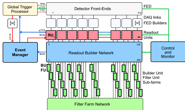
Figure 4: Sketch of the trapezoidal RU Builder.
