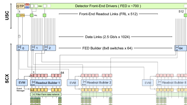
Figure 1: Sketch of the CMS DAQ system.
