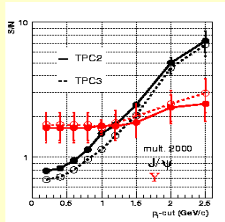
Signal/noise with p_T -cut
