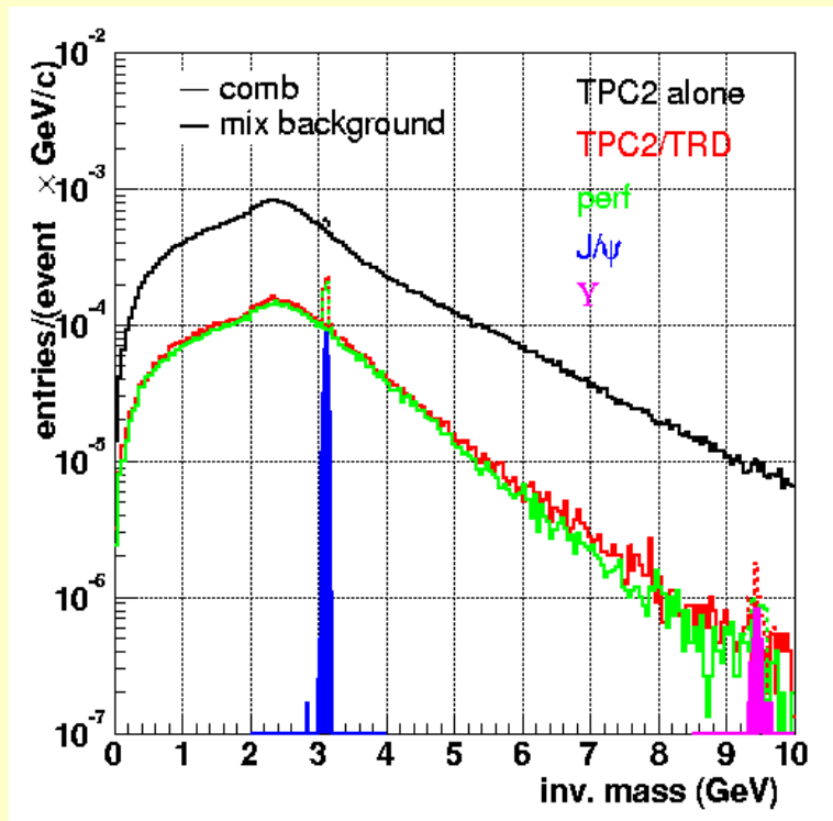
e^+e^- invariant mass
