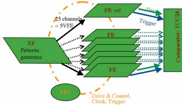
Figure 3: XFEST test bench
