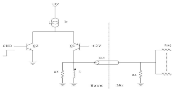
Figure 1: Pulser principle
