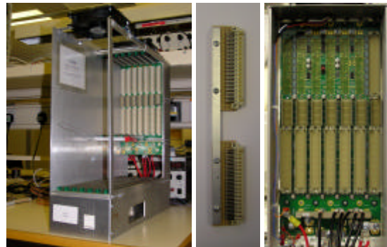
Figure 7: Boundary Scan crate and loop back cards.
