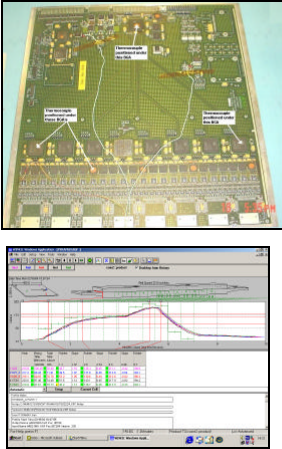
Figure 4: FED scrap board fitted with thermocouples and results from the re-flow oven profiling (courtesy DDi Technologies Limited).
