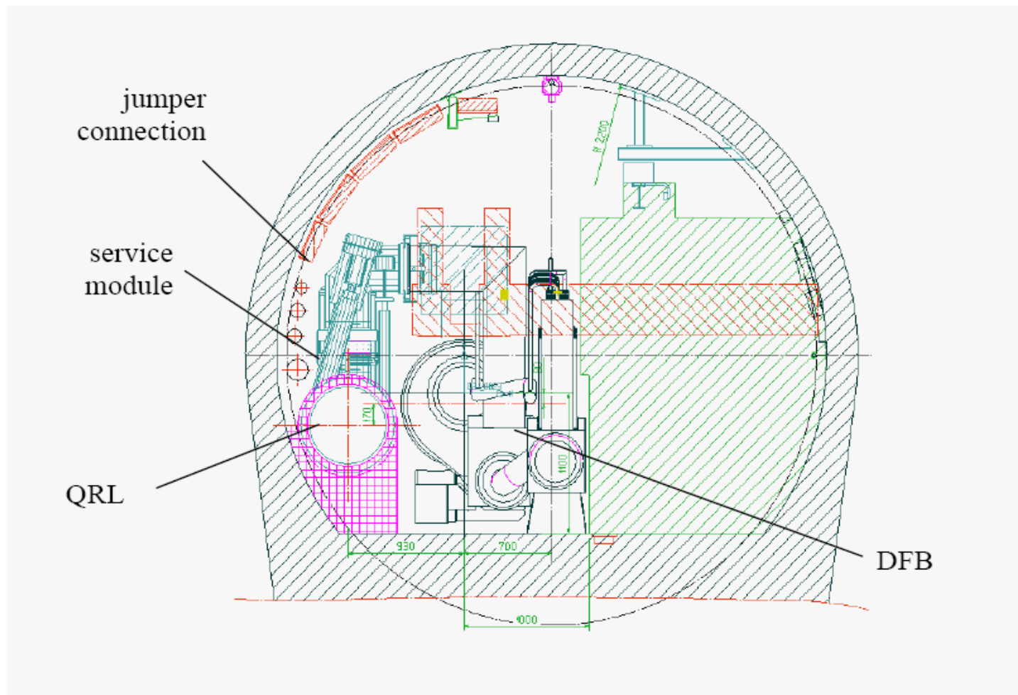
Figure 9.3: Enlarged tunnel cross section (RA) with DFBA
