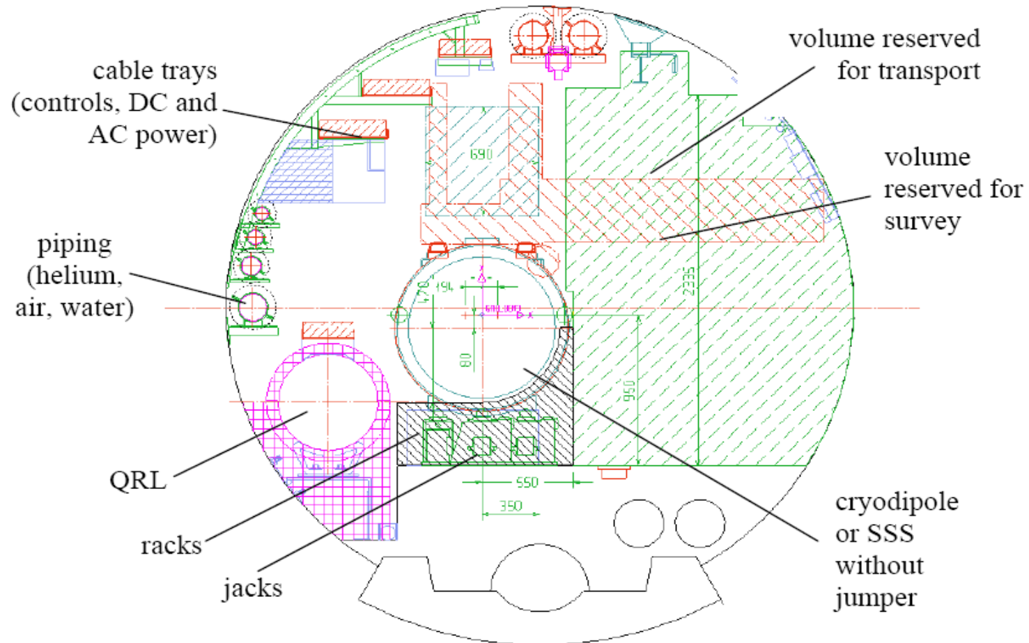
Figure 9.1: Standard Tunnel Cross section
