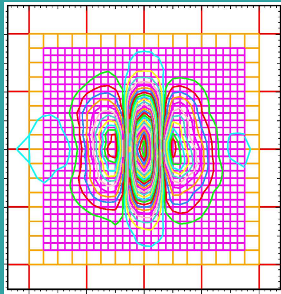
Density of secondary particles
