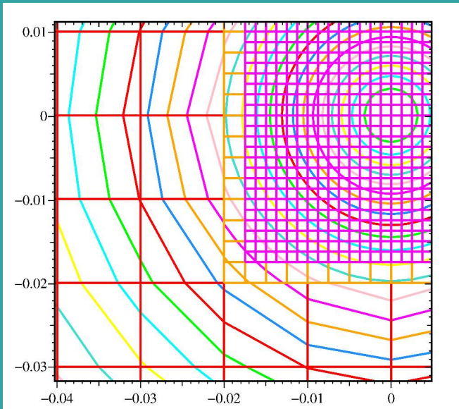
Electrostatic potential
