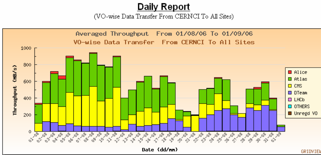
Figure 1 – Data distribution from CERN by VO – August 2006
