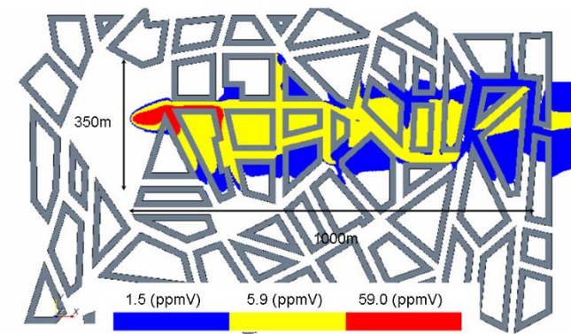
Full Navier-Stokes few hours or more
