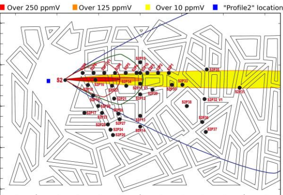
Gaussian
