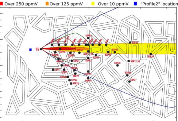
Gaussian few seconds
