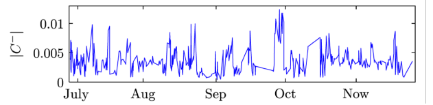
Figure 2: Coupling measurements made at injection throughout 2012 [11].
