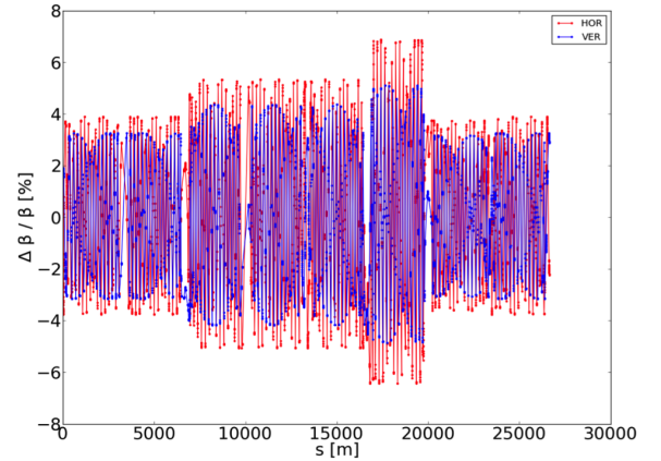
Figure 22: Horizontal (red) and Vertical (blue) beta-beating percentage due to beam-beam effects for a typical 2015 physics fill along the LHC circumference starting from IP3.
