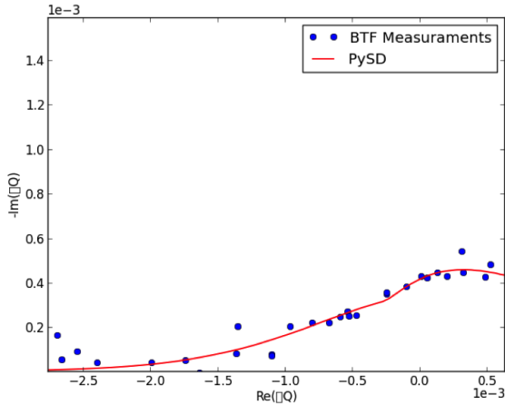
Figure 21: Computed (red line) versus measured (BTF reconstruction) stability diagram.
