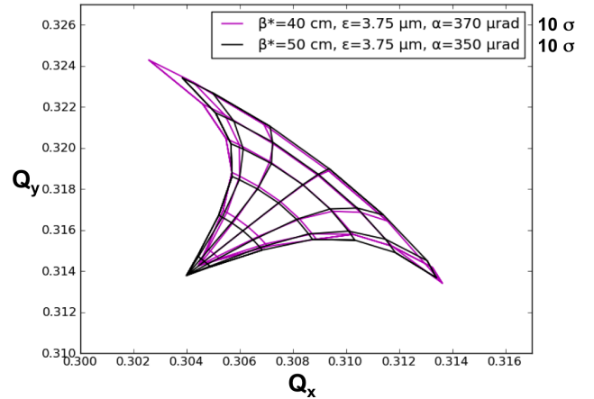
Figure 14: 2 Dimensional detuning with amplitude, footprint, for a separation of 10 \sigma in IP1 and IP5 for two possible optics the 40 (pink line) and 50 cm (black line).
