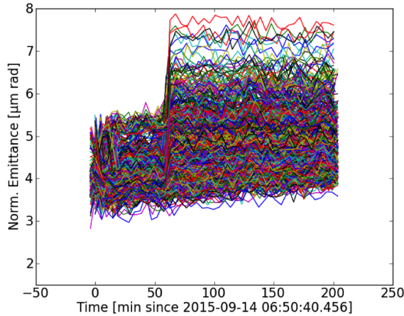
Figure 19: Bunch by bunch emittances in \mu\text{m} as a function of time during a physics fill of 2015 physics run. The emittances are measured by the BSRTs showing a sudden increase on selected bunches while beams were separated.
