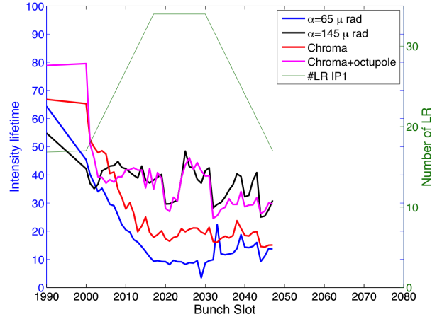
Figure 10: Beam 1 bunch by bunch lifetimes in hours as a function of the bunch slot position for the operational half crossing angle ( \alpha/2 = 145 \mu\text{rad} black line), for the reduced angle ( \alpha/2 = 65 \mu\text{rad} blue line), reduced chromaticity ( Q' reduced from 15 to 2 units, red line) and for reduced current in the octupole magnets (from 476 A to zero, pink line). The number of long-range encounters as a function of the 25 ns slot number are also shown (green line).
