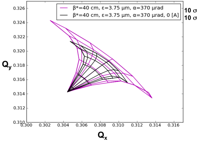
Figure 16: 2 Dimensional detuning with amplitude, footprint, for the 2016 physics run with (pink line) and without (black line) octupole magnets detuning.
