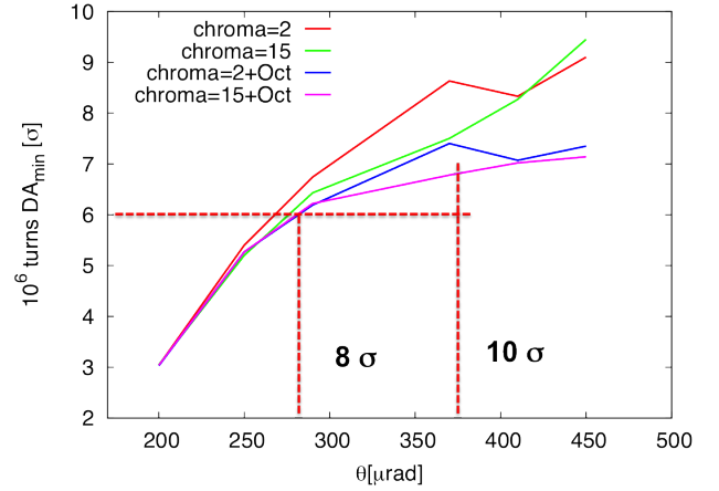
Figure 13: Dynamic aperture calculations as a function of the crossing angle \alpha in IP1 and IP5 for the 2016 LHC configuration: 40 \beta^* at the two IPs, bunch intensities of 1.3 \times 10^{11} protons and normalised transverse emittances of 3.75 \mu\text{m} . The different lines corresponds to beam-beam head-on and long-range interactions with chromaticity of 2 units (red line), with chromaticity of 15 units (green line), with octupoles at current of 550 A in positive polarity (blue line) and with chromaticity of 15 units and octupole at 550 A (pink line). The proposed crossing angle of 370 \mu\text{rad} corresponding to 10 \sigma beam to beam separation at the first long-range encounter is high lighted with the potential lower limit of 8 \sigma separation.
