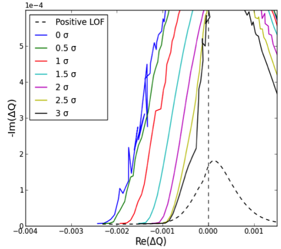
Figure 20: Horizontal (left) and Vertical Stability diagrams computed for a typical physics fill for different transverse separations at IP1 (legend). In dashed black lines the stability diagrams due to octupoles alone are plotted as a reference.
