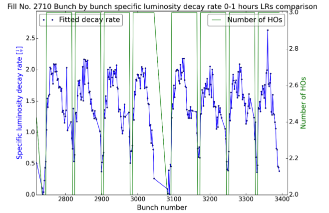
Figure 2: Bunch by bunch specific luminosity decay rate computed for first hour in stable beams during a representative physics fill number 2710 of the LHC physics fills of 2012.
