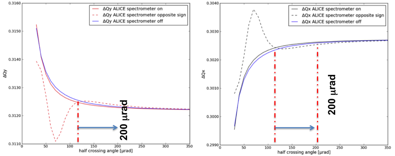
Figure 18: Vertical (left picture) and horizontal (right picture) tune shifted caused by the beam-beam effects at IP2 (the Alice experiment). The solid blue lines refer to the case without the spectrometer, red solid line to the case with spectrometer with polarity that sum up with the long-range beam-beam while the dashed line to the case with polarity that reduces the separation of the beam-beam encounters. The proposed half crossing angle to allow swap of spectrometer polarity is shown and is 200 \mu rad .
