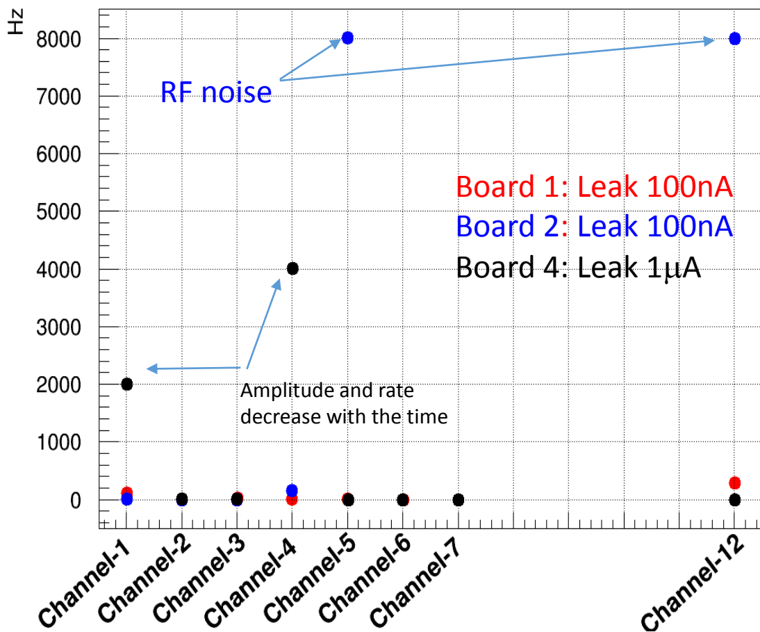
Noise Rate with 150 mV Trigger Threshold
