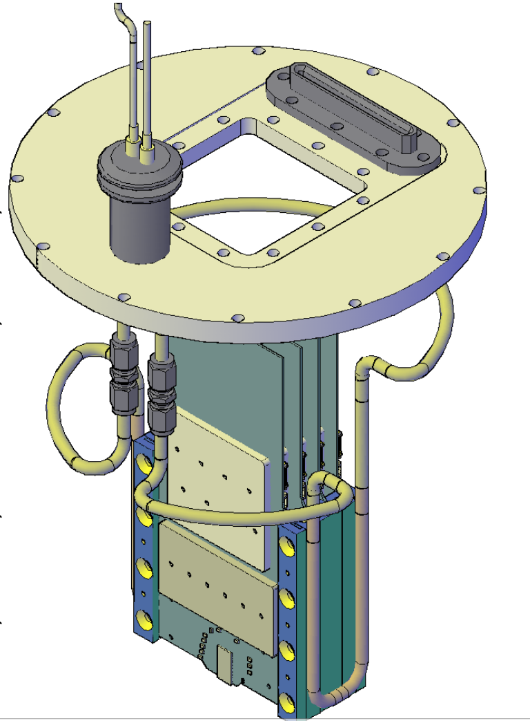
Final package of 4 diamond planes with its cooling system
