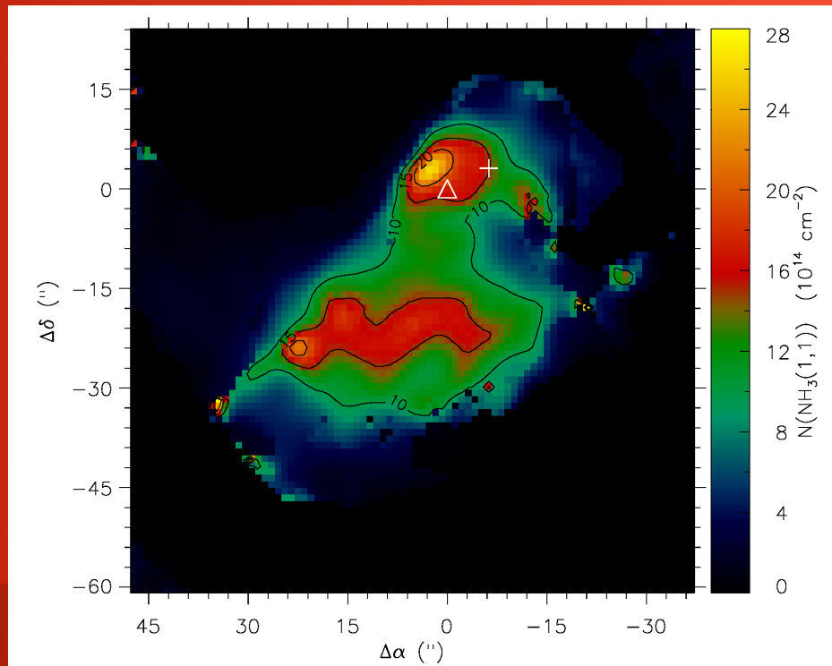
\text{NH}_3 observation of Chamaeleon-MMS1 Väisälä, Harju et al. (2014)
