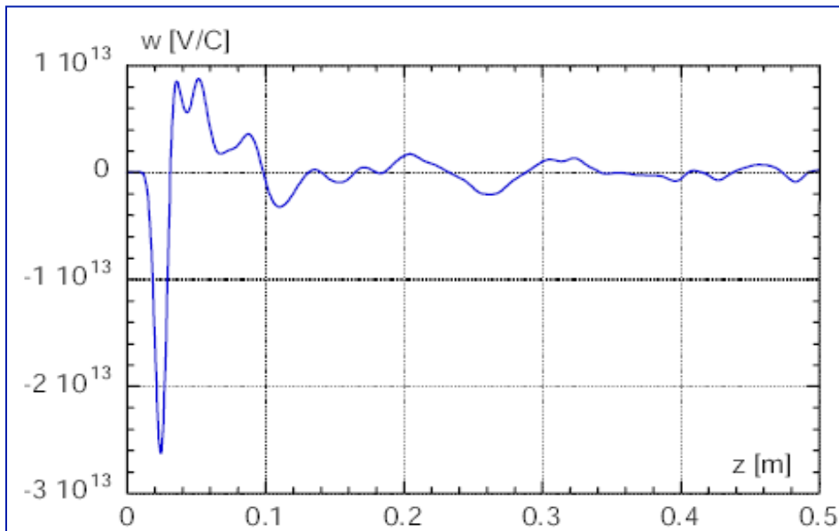
DAΦNE accumulator wake potential of a 2.5 mm Gaussian bunch.
