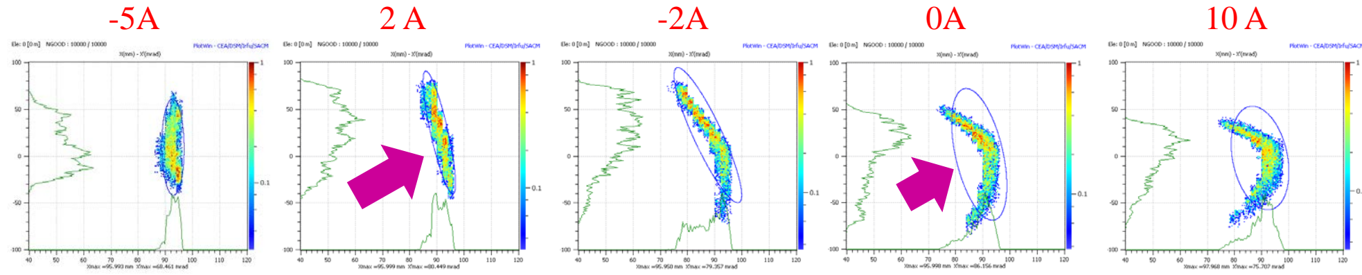
Horizontal emittance plot after the dipole vs current in the hexapole lens
