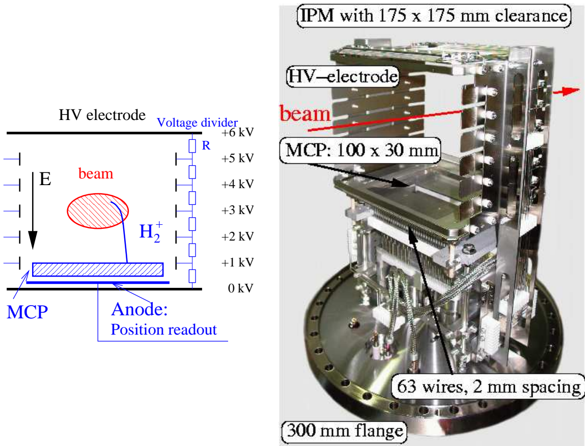
Figure 3.15: Left : Scheme of a ionization profile monitor for the horizontal profile determination. Right : The large aperture ionization profile monitor installed at the GSI synchrotron for the horizontal direction, the clearance is 175 \times 175 \text{ mm}^2 . The monitor is mounted on a \text{\O} 300 \text{ mm} flange. The read-out behind the MCP (bottom) is done with an array of 63 wires with 2 mm spacing.
