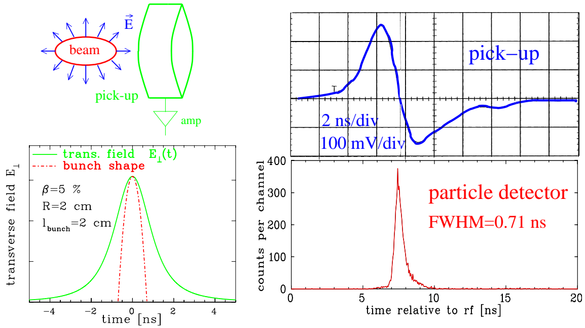
Figure 6.15: Left: Time evolution of transverse electric field as seen by the pick-up is simulated for the for a bunch with \cos^2 -distribution. Right: The comparison of a pick-up signal to the bunch structure measured with a particle detector at the GSI LINAC with 1.4 MeV/u. The broadening of the pick-up signal due to the longitudinal field component is clearly visible.
