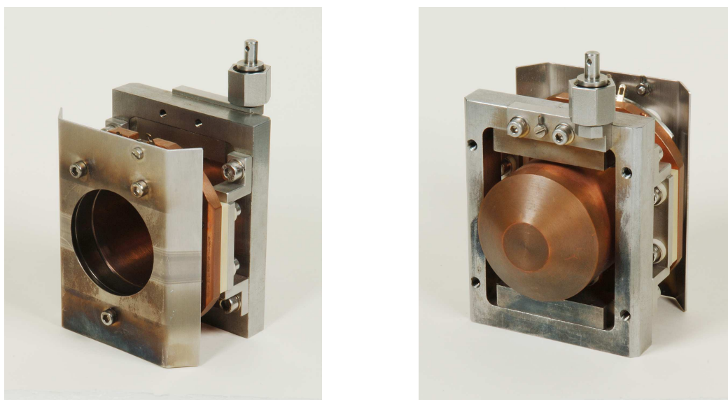
Figure 2.22: Photo of an Ø50 mm uncooled Faraday cup with magnetic and electric secondary electron suppression.
