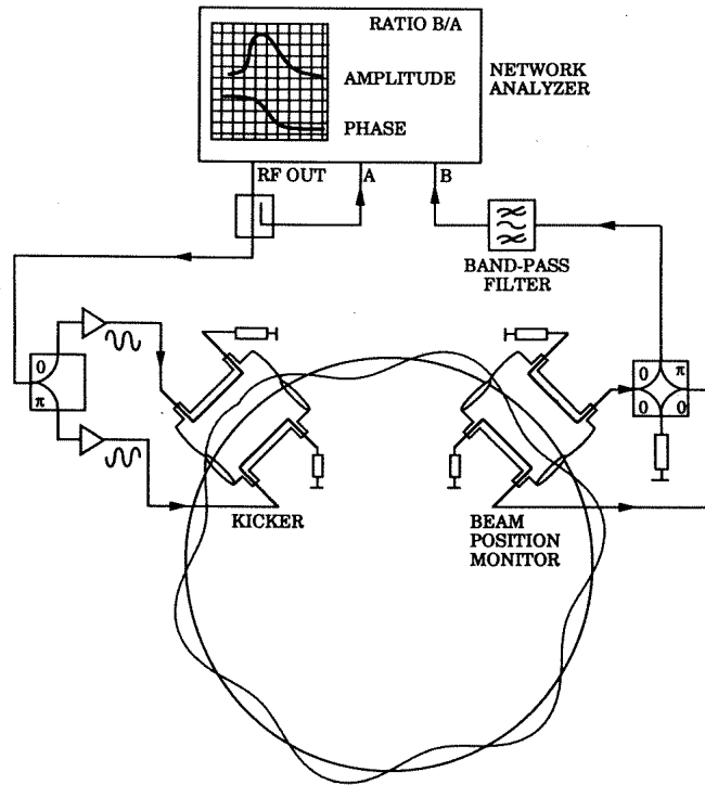
Figure 5.33: Scheme of a beam transfer function (BTF) measurement.
