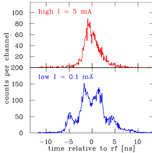
Figure 6.21: The bunch structure measured at the GSI LINAC with a 120 keV/u \text{Ar}^{1+} beam for different currents inside the RFQ [74]. The influence of the beam's space-charge to the longitudinal emittance is demonstrated by it. One rf-period is shown.
