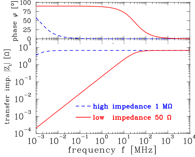
Figure 5.3: Absolute value and phase of the transfer impedance for a l = 10 cm long cylindrical pick-up with a capacitance of C = 100 pF and an ion velocity of \beta = 50\% for high ( 1 \text{ M}\Omega ) and low ( 50 \Omega ) input impedance of the amplifier. The parameters are typical for a proton or ion synchrotron. The high-pass characteristic is clearly seen corresponding to a signal decreasing for low frequencies.
