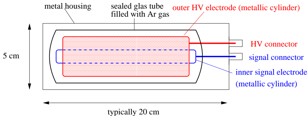
Figure 8.7: Scheme of an ionization chamber as used for beam loss detection.
