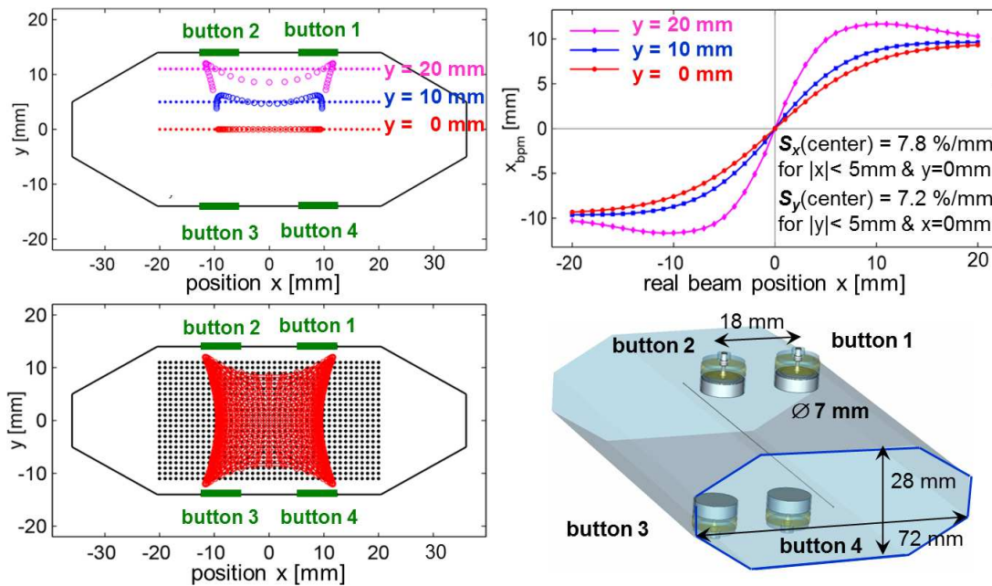
Figure 5.16: Numerical calculation of the position map for the arrangement at the synchrotron light source ALBA. Top left: Results of position calculation for a horizontal scan from -20 \text{ mm} < x < 20 \text{ mm} for three vertical offsets using constant horizontal S_x(\text{center}) and vertical S_y(\text{center}) position sensitivities. Top right: The calculated position for the horizontal scan for these three vertical offsets; the horizontal position sensitivity S_x(\text{center}) at the central part is determined from the slope of the curve with zero vertical offset. Bottom left: Position map for the entire horizontal and vertical range. Bottom right: The geometry of the \text{\O} 7 \text{ mm} button pick-ups of 18 mm horizontal distance within the chamber; from [90].
