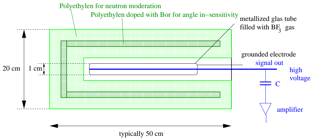
Figure 8.6: Scheme of a \text{BF}_3 proportional tube as used for beam loss detection. The proportional tube is filled with \text{BF}_3 gas surrounded by polyethylene for the moderation of the neutrons.
