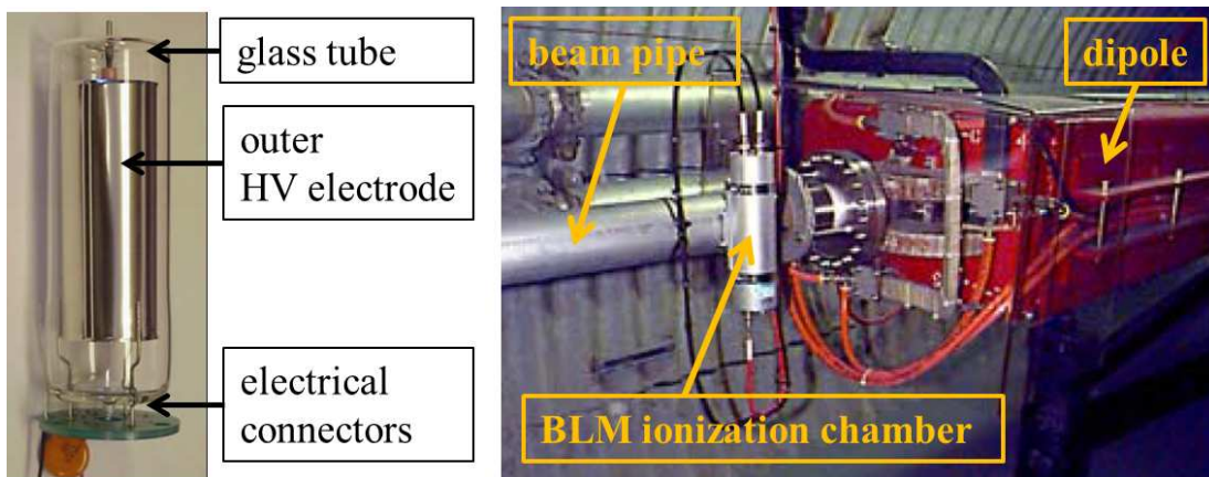
Figure 8.8: Left: Photo of an co-axial ionization chamber use as a beam loss monitor. Right: The installation of such a ionization chamber for beam loss detection in a transport line.
