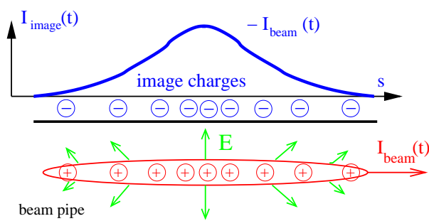
Figure 5.1: The beam current induces a wall current of the same magnitude and time structure but reversed polarity.
