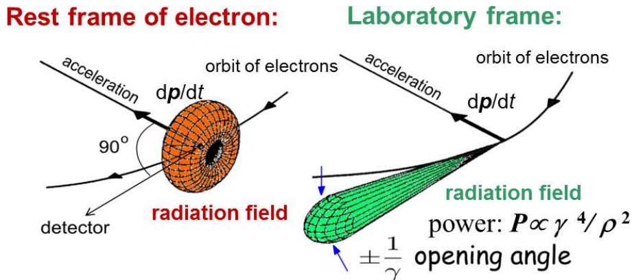
Figure 3.26: Forward peaked synchrotron radiation for relativistic particles from a bending magnet.
