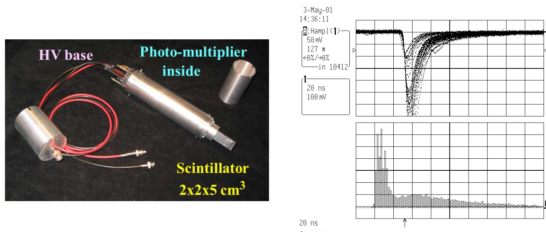
Figure 8.4: Left. Photo of a typical BLM based on a plastic scintillator connected to a photo-multiplier. Right: Typical pulses from a plastic scintillator (top, 100 mV/div and 20 ns/div) and their pulse height distribution (bottom, 50 mV/div) as measured at the GSI heavy ion synchrotron.
