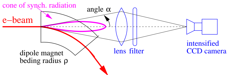
Figure 3.27: Scheme for a synchrotron radiation profile monitor observing the radiation from a dipole.
