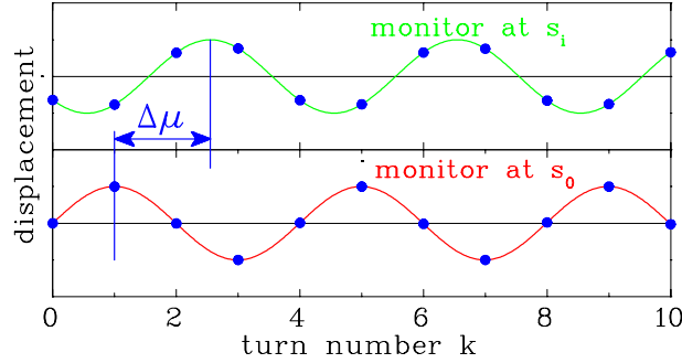
Figure 5.36: Scheme of the individual measurements at two pick-ups for a phase advance \Delta\mu determination. A sine function can be fitted through the data points.
