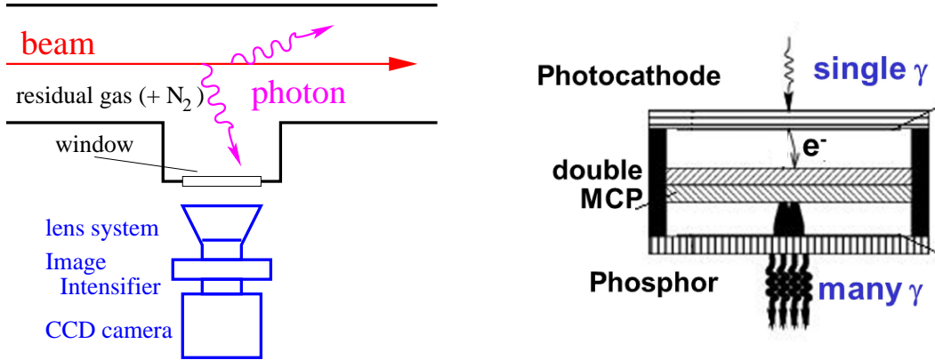
Figure 3.21: Left: General scheme of the profile determination via detection of the residual gas fluorescence. Right: Scheme of an image intensifier consisting a photo-cathode, a MCP and a phosphor screen.
