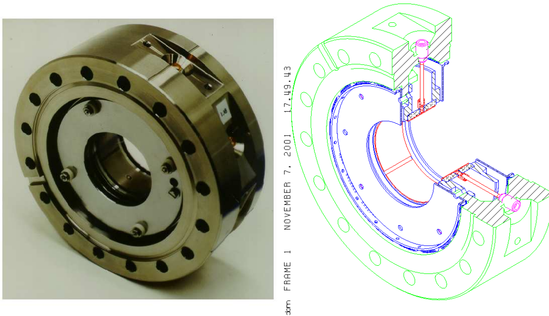
Figure 5.10: Photo and schematic drawing of a capacitive position sensitive pick-up at the GSI-LINAC. The aperture is 50 mm and the electrode length 20 mm.
