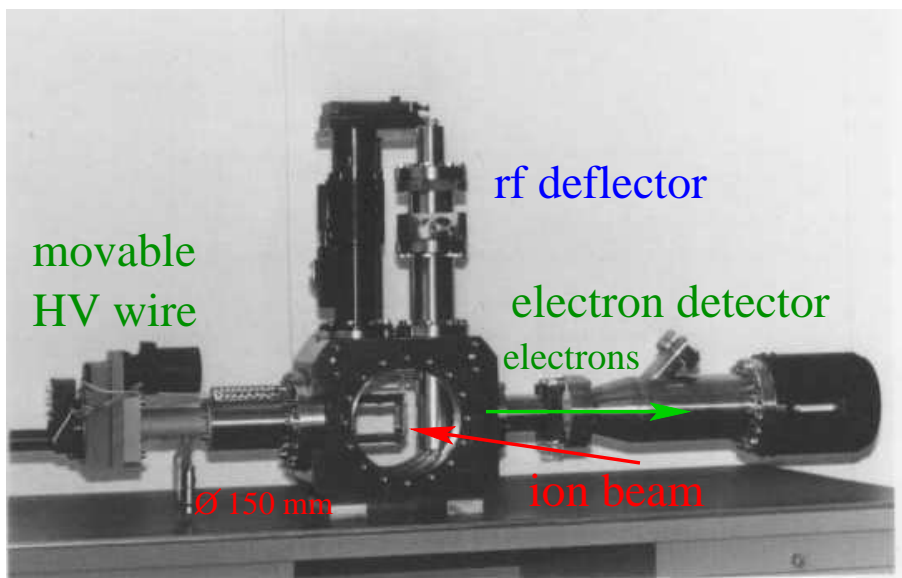
Figure 6.24: The bunch shape monitor (BSM) installed at CERN LINAC 2 [122]. The vacuum feed-through on the left side is the support for the high voltage wire. The rf-deflector is installed on the vertical flange and the detector is mounted on the right.
