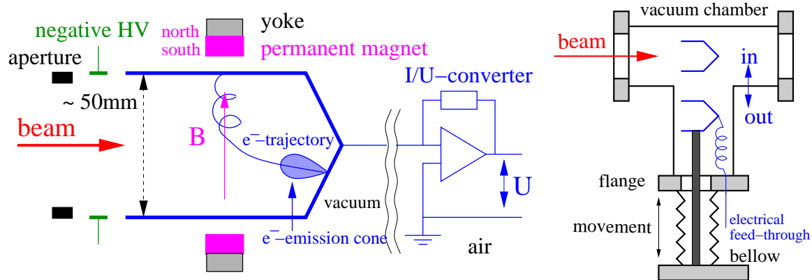
Figure 2.21: Left: Scheme of an uncooled Faraday cup with magnetic and electric secondary electron suppression. Right: Scheme for inside and outside position of destructive diagnostics devices.
