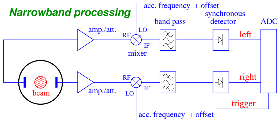
Figure 5.25: Schematic signal analysis for a narrowband treatment.
