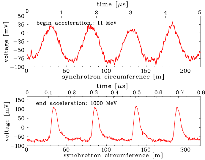
Figure 5.5: Bunch signals from a shoe-box pick-ups for 1 M \Omega termination as installed at the GSI ion synchrotron. The upper curve shows the bunches along the synchrotron circumference at the begin of the acceleration, the lower curve after reaching the final energy. Note the different time scales on top of the plots.
