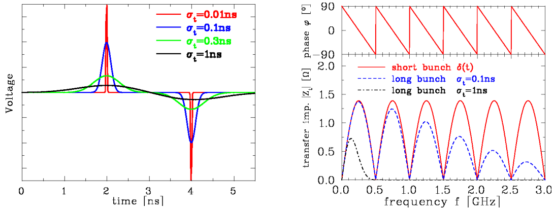
Figure 5.22: Calculation of a voltage signal at the upstream port of a stripline BPM of l = 30 cm and a coverage of \alpha = 10^\circ for different bunch durations \sigma_t (left) and the corresponding transfer impedance (right).
