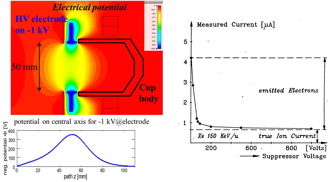
Figure 2.23: Left: The electric potential of the Faraday cup shown in Fig. 2.22 with the high voltage electrode biased by -1 kV is shown at the cylindrical symmetry plane. The beam enters from left. The negative potential along the central axis is depicted at the bottom. Right: The effect of secondary electrons suppression inside a Faraday cup as determined by the beam current determination a function of applied voltage.
