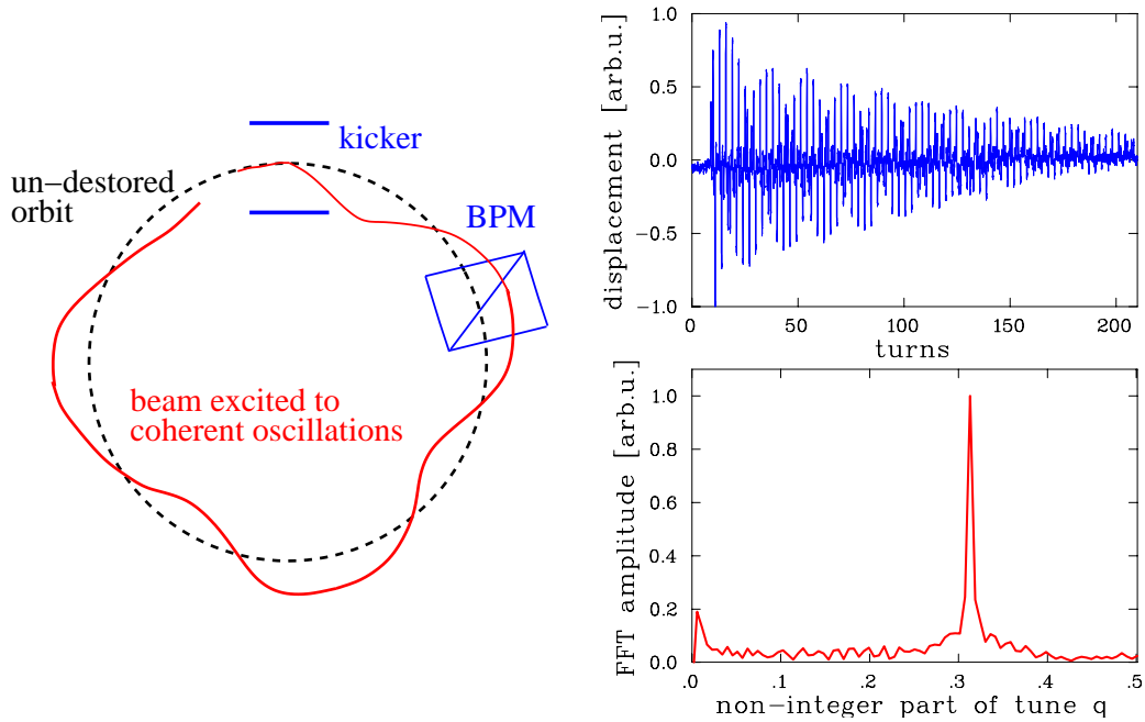
Figure 5.31: Left: Scheme of the beam excitation and detection of coherent bunch oscillations by a BPM. Right: Beam oscillations after a kick excitation recorded in the time domain for 200 turns (top) and its Fourier transformation for q determination (bottom) at the GSI synchrotron.
