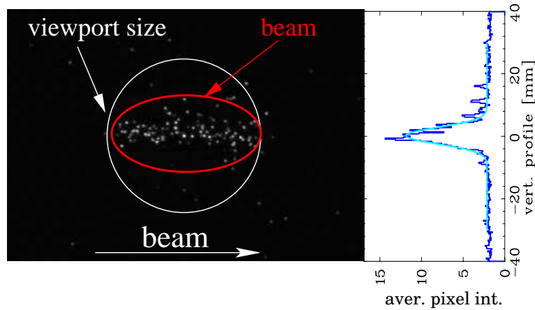
Figure 3.23: Image of a 250 \mu\text{s} \text{Ar}^{10+} beam of I_{\text{beam}} = 2.5 \text{ mA} and a vacuum pressure of 10^{-5} \text{ mbar} recorded at the GSI LINAC. The original image (recorded with a double MCP intensifier) is shown and the projection for the vertical profile [54].
