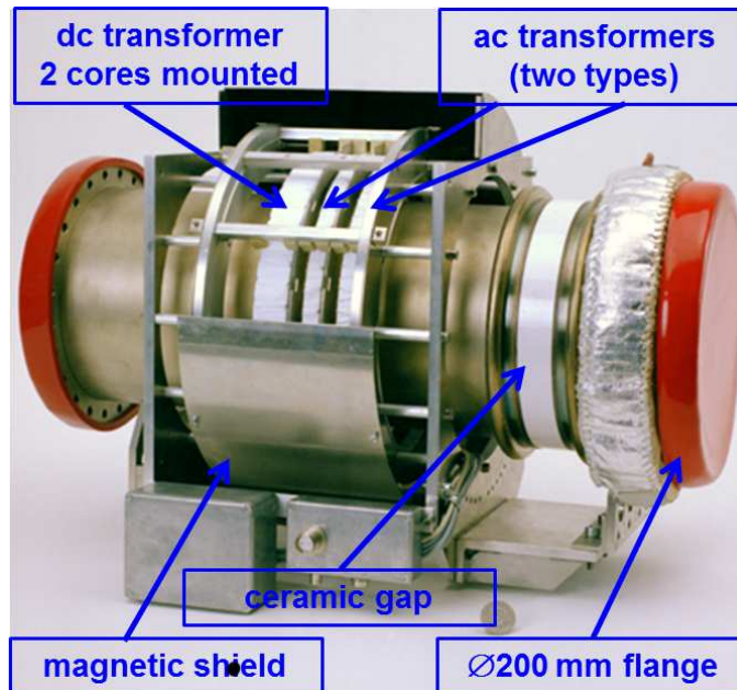
Figure 2.15: The dc-transformer installed at the GSI synchrotron. The left torus is the dc-transformer (two tori mounted closely together), the middle is the ac-transformer used for the feedback of the dc-type and the right one is the ac-transformer for the control of the injection.
