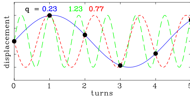
Figure 5.30: Schematic of the tune measurement for six subsequent turns determined with one pick-up, together with with the three lowest frequency fits.
