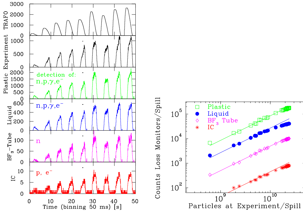
Figure 8.10: Left: Typical example from different beam loss monitors for a O^{8+} beam accelerated from 11 to 800 MeV/u for nine cycles with varying intensities up to 4 \times 10^{10} particles per cycle [138]. Right: Linearity of the loss monitors as a function of the current for the same parameters. The lines are linear fits.
