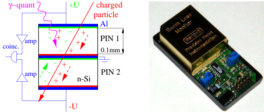
Figure 8.5: Scheme of a two PIN diodes driven in coincidence and a photo of the device [5].
