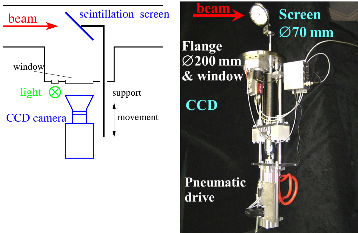
Figure 3.1: Scheme of a intercepting scintillator screen is shown left. On the right a photo from a P43 phosphor scintillation screen of \text{\O}70 mm and the CCD camera are mounted on a \text{\O}200 mm flange with pneumatic feed-through is depicted.
