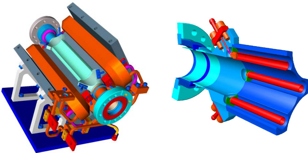
Figure 5.23: Technical drawing of the stripline BPM installed inside a quadrupole magnet at TTF2 (left) and the design of the transition for the strip to the feed-through (right). The beam pipe has \text{\O} 34 mm, from [93, 94].
