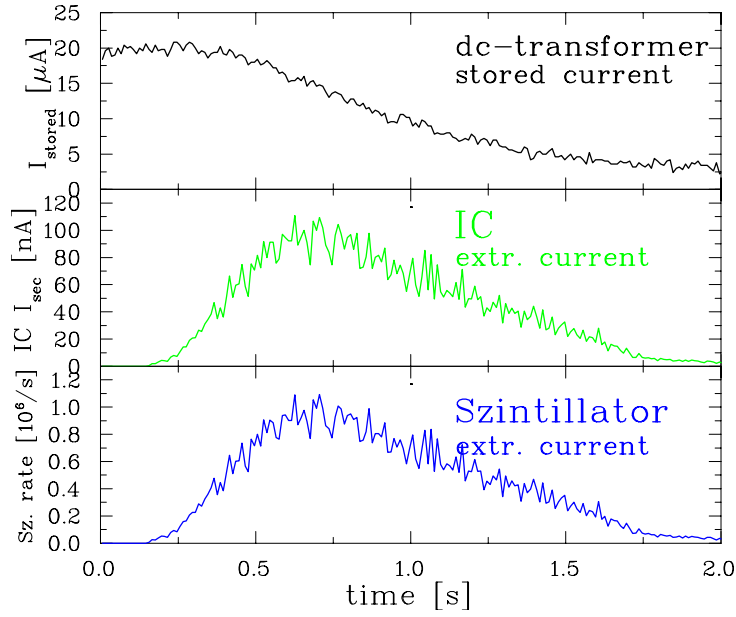
Figure 2.34: The extracted current measured with an IC (middle, given in nA for the secondary current) and a scintillator (bottom, given in particles per second) as compared to the current inside the GSI synchrotron determined by dc-transformer (top, given in \mu\text{A} ) for one extraction of a 250 MeV/u ^{208}\text{Pb}^{67+} beam with a total amount of 10^6 particles.
