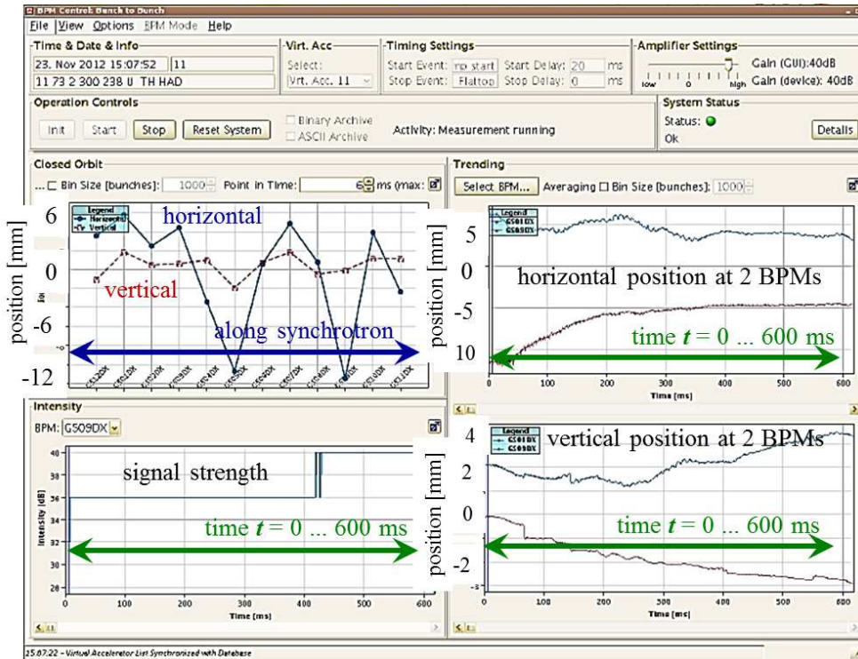
Figure 5.29: Example of a position measurement done at the GSI synchrotron for a partly misaligned beam during a 0.6 s long acceleration. The upper left top plot shows the position around the ring at 12 locations at the begin of the ramp; the upper right plot shows the horizontal position during the acceleration ramp for two BPM locations, the lower right plot the vertical position for these BPMs; the lower left plot is a signal power \propto U_{\Sigma}^2 during the ramp for the a single BPM. The panel at the top is used for the control of pre-amplifiers and for timing.
