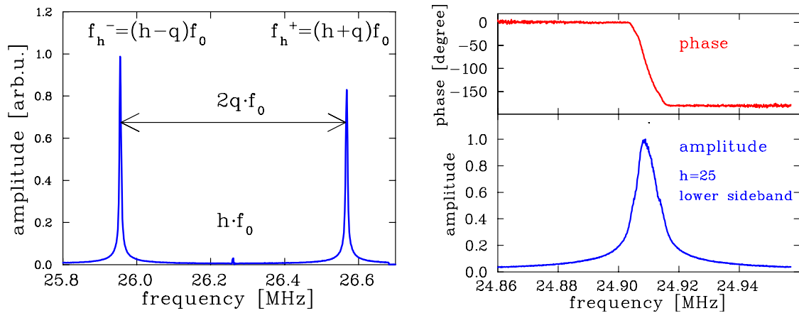
Figure 5.34: BTF measurement at the GSI synchrotron with a 500 MeV/u U^{73+} beam having a revolution frequency of f_0 = 1.048 MHz. The wide scan around the h = 25^{th} -harmonics is shown left and a scan around the lower sideband centered at f_{25}^- on the right. The fractional tune is q = 0.306 for these data.
