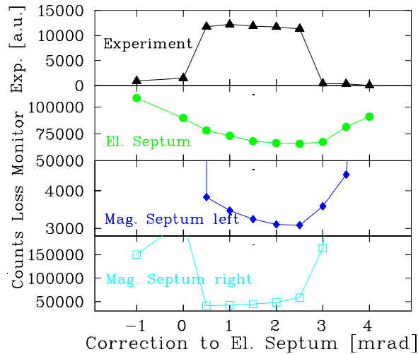
Figure 8.12: Counts per spill from three loss monitor locations and the current at the experiment as a function of the angle electrostatic septum at the GSI synchrotron [138].
