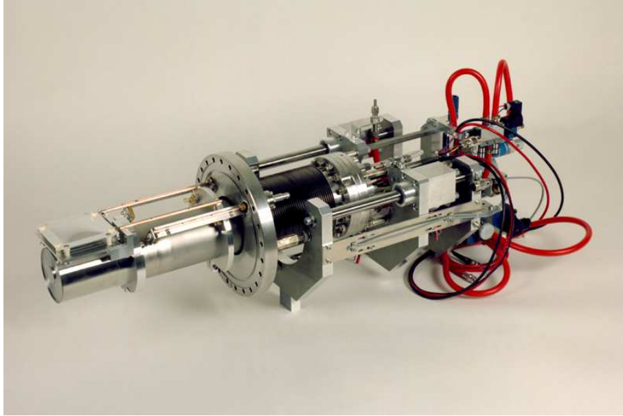
Figure 2.35: The feed-through mounted on a \text{Ø}200 mm flange containing the scintillator and IC inside the pocket at atmospheric pressure and the SEM in the vacuum.
