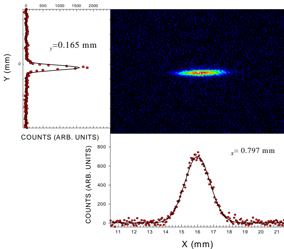
Figure 3.30: Image of the electron beam in the APS accumulator ring (Argonne National Lab.) by a synchrotron radiation monitor [66].
