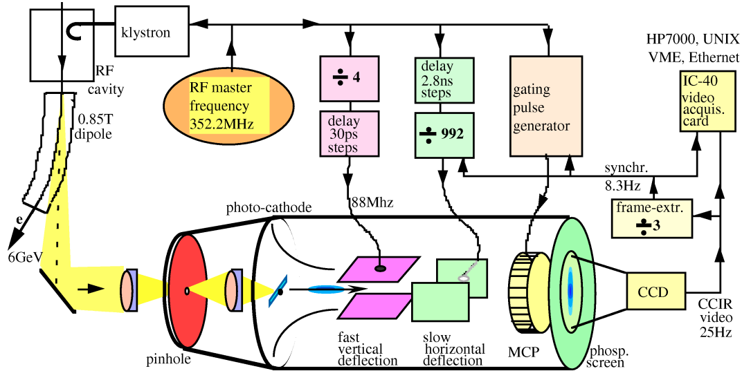
Figure 6.25: Principle of a streak camera measurement for bunch width determination at electron accelerators ESRF, from [126].
