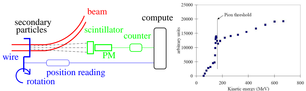
Figure 3.10: Left: Scheme of a wire scanner using the production of secondary particles as the signal source. Right: The total rate from a wire scanner under proton impact at CERN PS-Booster, showing the rate increase above the \pi -threshold at \sim 150 \text{ MeV} , from [37].
