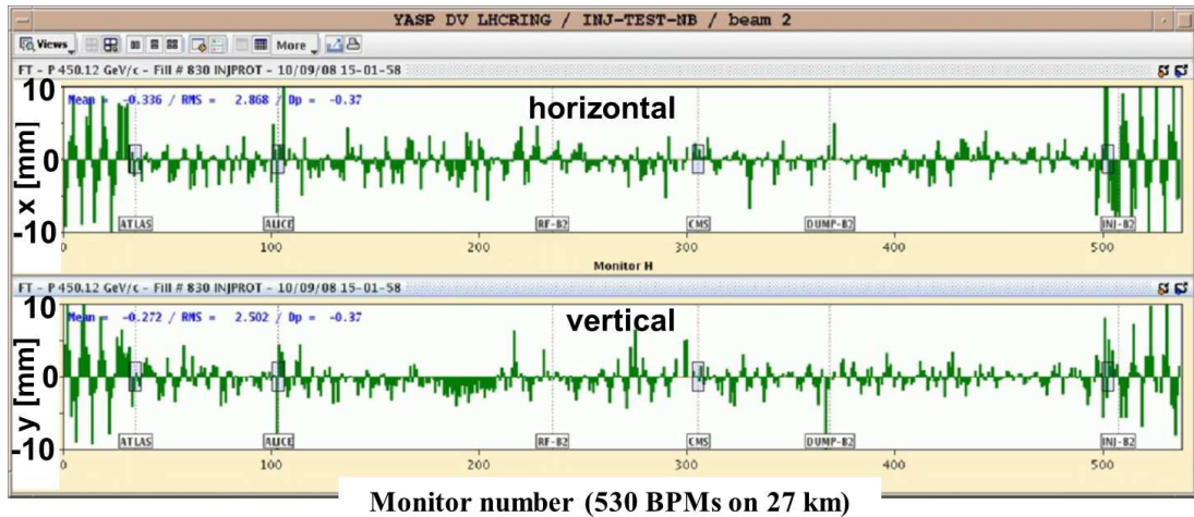
Figure 5.28: Measurement of the trajectory of a single bunch injected in the LHC with a position display at the 530 BPMs around the synchrotron, from [103].
