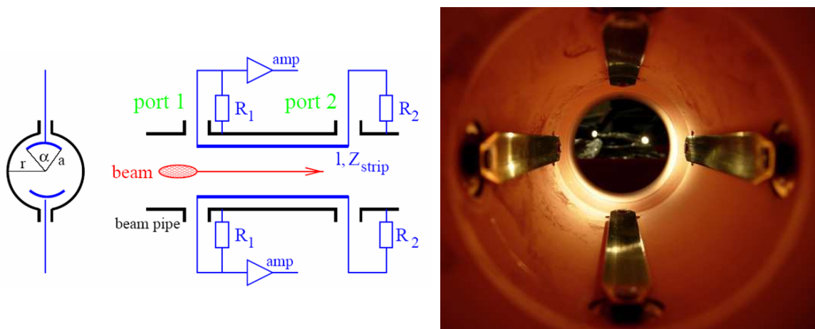
Figure 5.20: Left: Scheme of a stripline pick-up. Right: Photo of the LHC stripline BPM of 12 cm length, from [86].
