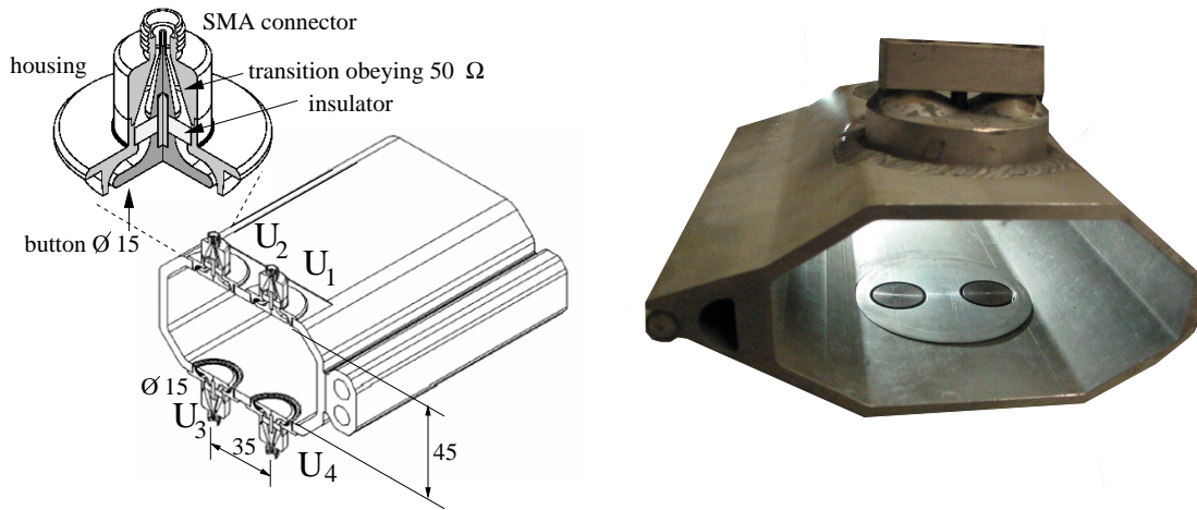
Figure 5.15: Left: Typical button BPM arrangement within a vacuum chamber at a synchrotron light source, from [87]. Right: Photo of the realization at HERA, DESY.
