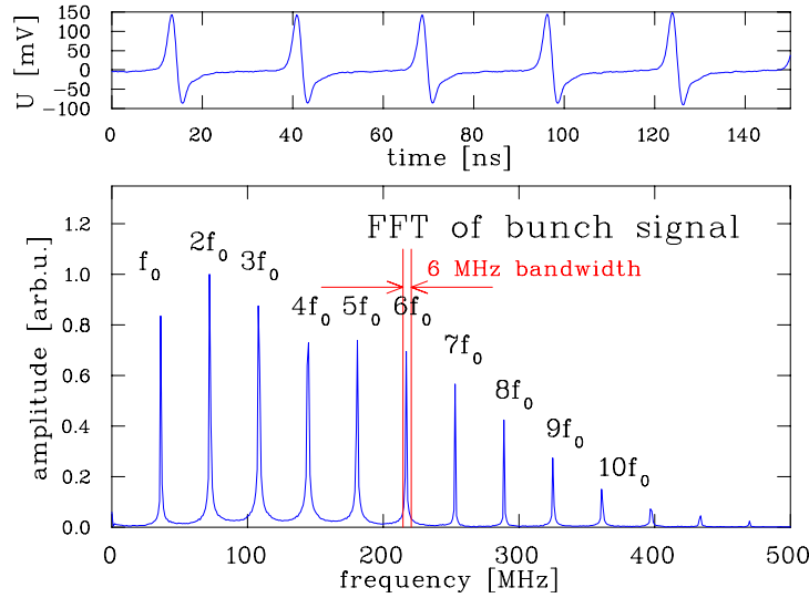
Figure 5.26: Bunch signal (top) and its Fourier transformation (bottom) at the GSI-LINAC of a 1.4 MeV/u beam. In the Fourier spectrum each line corresponds to the indicated harmonics of the 36 MHz accelerating frequency. The position evaluation is done at 6f_0 = 216.8 MHz by a 6 MHz narrowband processing as indicated by the red lines.
