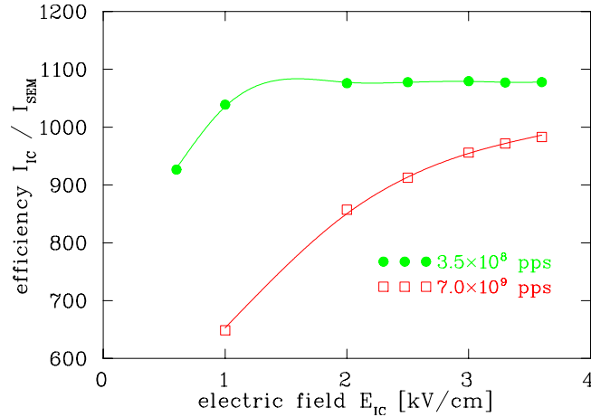
Figure 2.38: The characteristic line for the IC as determined of the 300 MeV/u Ne 10+ beam. The efficiency, as measured by the ratio of the secondary current of the IC and the SEM as a function of the applied electric field [16]. For a low primary current a plateau is reached, while for a high current the recombination leads to a decrease of the secondary charges.
