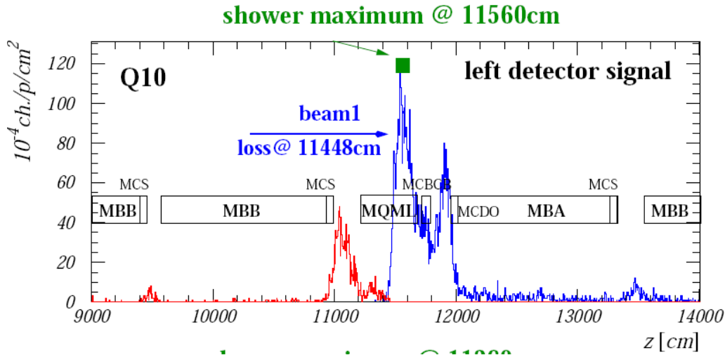
Figure 8.11: Simulation of a secondary particle distribution (hadron shower) due to a proton loss inside a quadrupole for the LHC and 7 TeV protons [143]. The maximum of the shower is about 1 m from the loss point.
