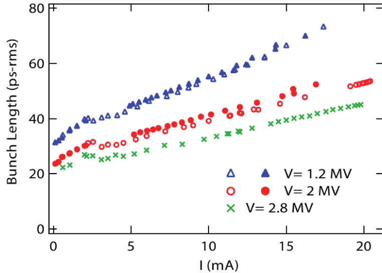
Figure 6.27: Example of the use of a streak camera at the synchrotron light facility SOLEIL achieved from measurements like depicted in Fig 6.26: For different accelerating voltages the bunch length is recorded as a function of the beam current stored in the synchrotron, from [127]. [127].
