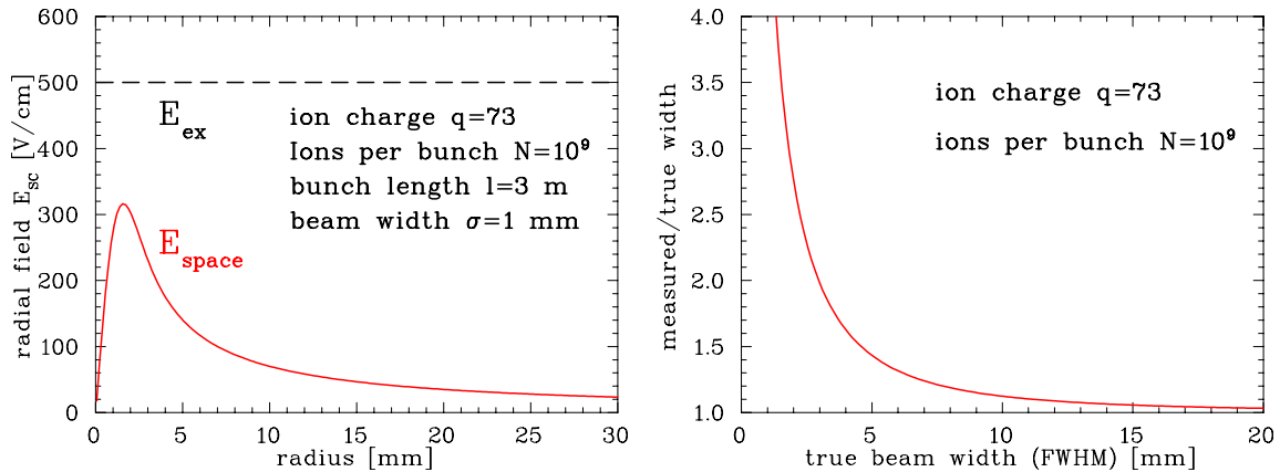
Figure 3.19: Model calculation of the beam broadening due to the space charge field of a U 73+ with 10 9 particles per 3 m bunch length (left). The resulting relative broadening using an ionization profile monitor with ion detection (right) is plotted for this current. The parameters are valid for an intense, cooled ion beam.
