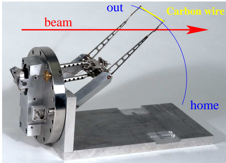
Figure 3.9: Pendulum scanner or 'flying wire' used at CERN synchrotron [35].
