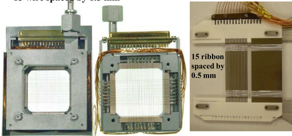
Figure 3.4: Left: SEM-grid for both planes with 15 tungsten wires spaced by 1.5 mm as typically used at a proton LINAC. The individual wires are insulated with glass-ceramics. Right: SEM-grid based on ribbon made from 25 \mu\text{m} thick aluminium foil by laser cutting; the spacing is 0.5 mm. This type is used for high energetic proton above typically 1 GeV. The devices are mounted on a pneumatic feed-through to move it in and out of the beam (not shown).
