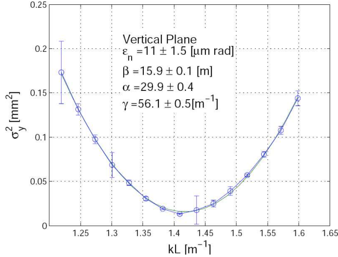
Figure 4.9: Profile width determined with a YAG:Ce screen at Elettra electron LINAC for a quadrupole variation and the parabolic fit, from [75].
