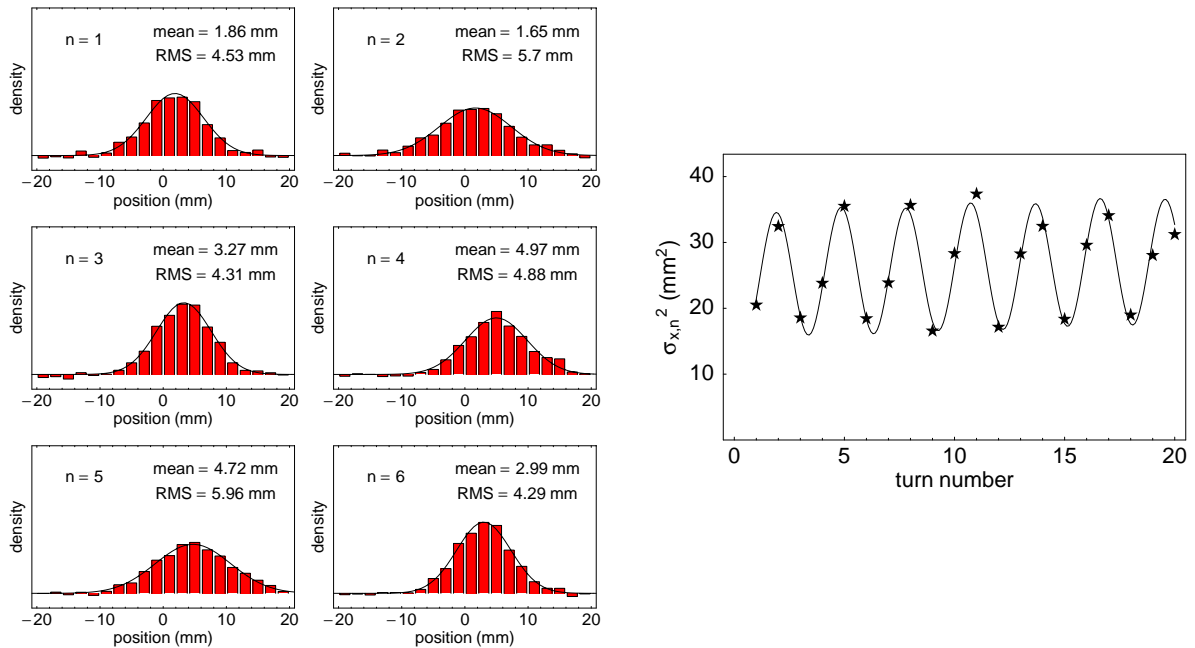
Figure 3.8: Profile measurement for a mismatched injection into the CERN PS synchrotron for the first n = 1 \dots 6 turns and the fitted square of the beam width as a function of time, from [41].
