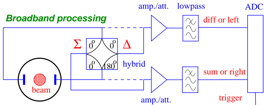
Figure 5.24: Scheme of a broadband signal processing. The plate signals are either fed directly to the amplifier (dashed line) or via a hybrid the sum and difference is generated in an analog manner (solid line).
