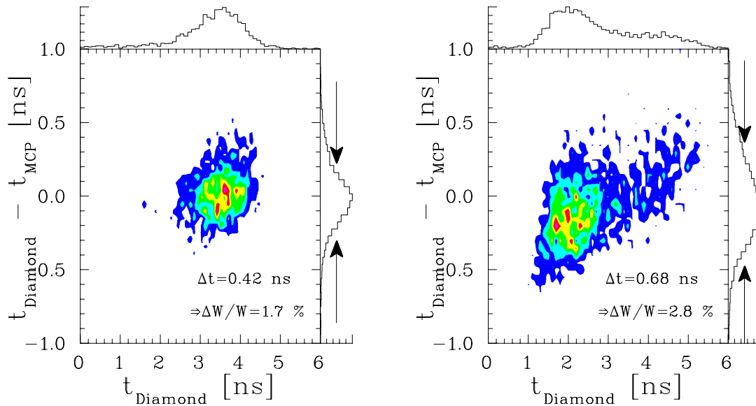
Figure 6.22: Phase space plot for a 1.4 MeV/u ion beam recorded with two detectors in coincidence at the GSI LINAC [74]. The time relative to the rf is plotted along the horizontal axis, the time difference of the individual particles on the vertical axis corresponding to the energy distribution. The low current ( I_{beam} = 0.1 mA) results are plotted left. For a high current beam ( I_{beam} = 5 mA) the emittance is asymmetrically broadened by space charge forces (right).
