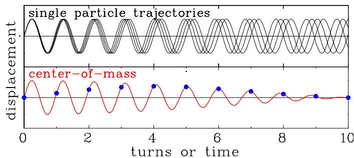
Figure 5.32: Plot of the individual trajectories of four particles after a kick (top) and the resulting coherent sum signal as measured by a pick-up (bottom). (The tune spread is much to large for a real machine.)
