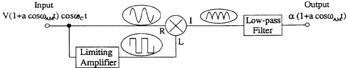
Figure 5.27: Scheme of a synchronous detector to rectify an rf signal: The rf signal is split and one branch is fed into a limiter amplifier driven into saturation, which transforms the signal to a bipolar rectangular pulse. This signal is mixed with the original signal to yield a unipolar waveform (corresponding to the square). It is passed through a low-pass filter and can then be digitized by a low sampling ADC.
