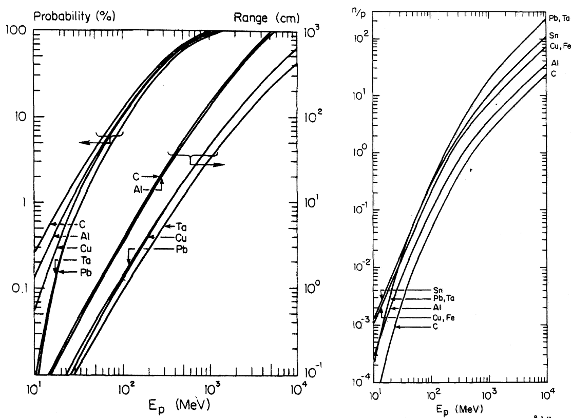
Figure 8.2: Left: The ranges of protons in various metals and the probability of an inelastic nuclear reaction within the range as a function of the proton energy, i.e. within a thick target. Right: The total number of neutrons per proton incident on a thick target of various metals as a function of the proton energy, from [136].
