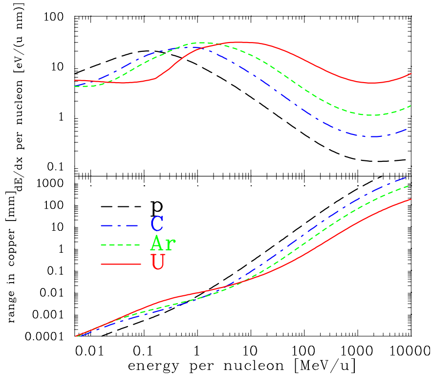
Figure 2.18: The energy loss per nucleon at the surface and the range in copper as a function of the kinetic energy for several ions. The energy range is plotted from 5 keV/u to 10 GeV/u and the range from 100 nm to 1m. The calculation of the electronic and nuclear stopping uses the semi-empirical code SRIM [13].
