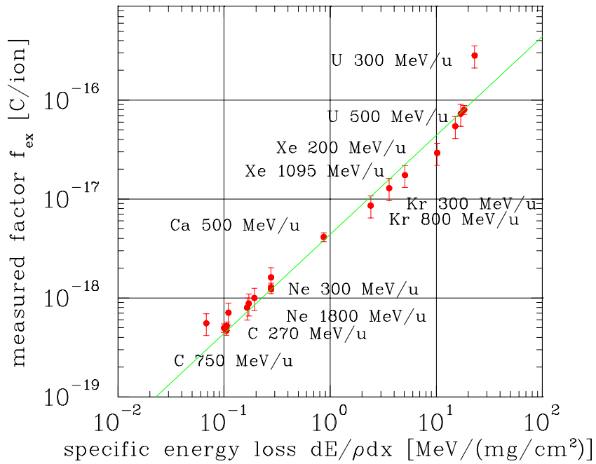
Figure 2.40: The measured calibration factor of a SEM and calculated value using energy loss and a fitted value of Y = 27.4 e^-/(\text{MeV}/\text{mg}/\text{cm}^2) for various slowly extracted ion from the GSI synchrotron [17].
