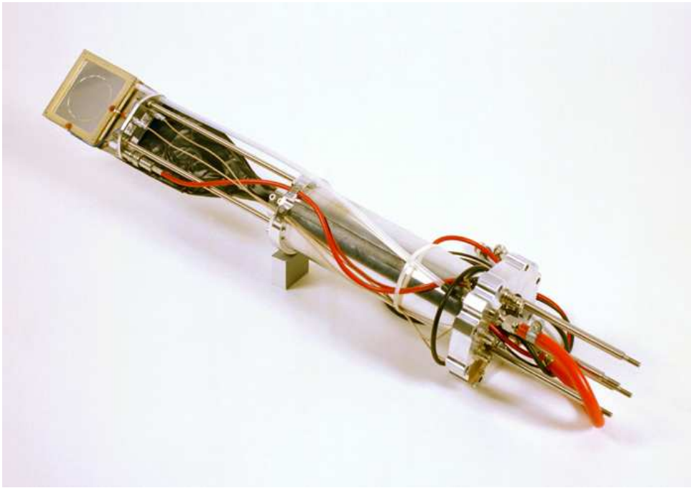
Figure 2.32: The hardware of the scintillators (wrapped in black tape) and the IC installed at GSI.
