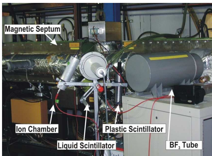
Figure 8.3: The tested beam loss detectors installed at the extraction from the GSI heavy ion synchrotron [138].
