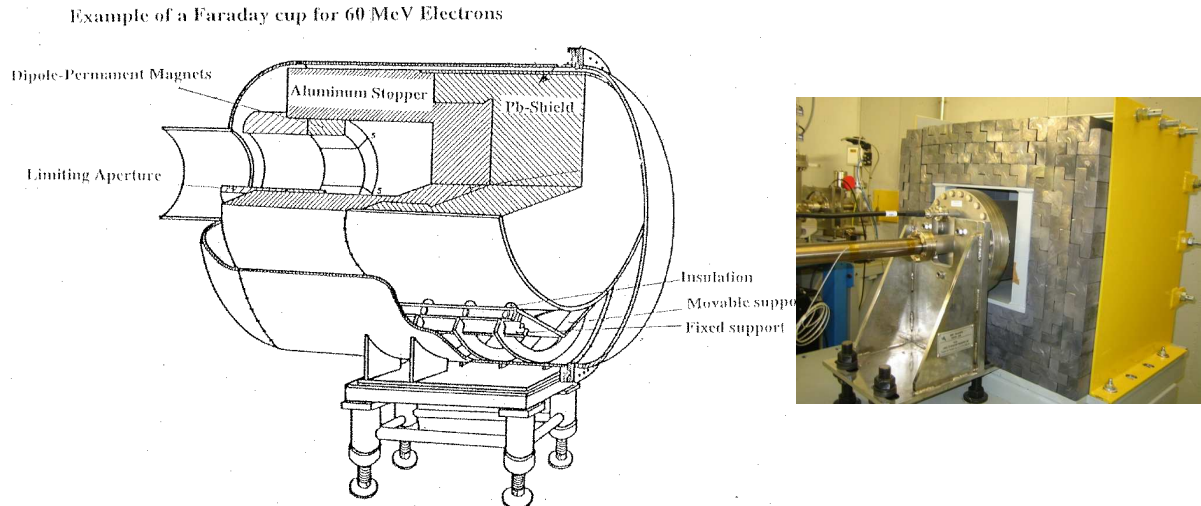
Figure 2.29: Left. A drawing of a cup used for 60 MeV electrons. Right. The installation of a Faraday cup used as a beam dump at ALBA, Barcelona.
