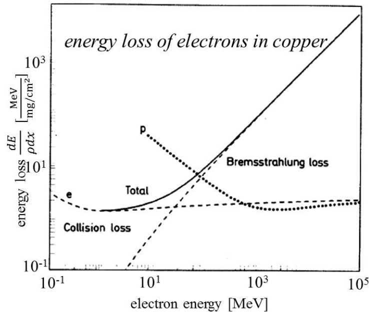
Figure 2.19: The energy loss of electrons in copper for collision and radiation losses [10]. For comparison the loss of protons are also shown.
