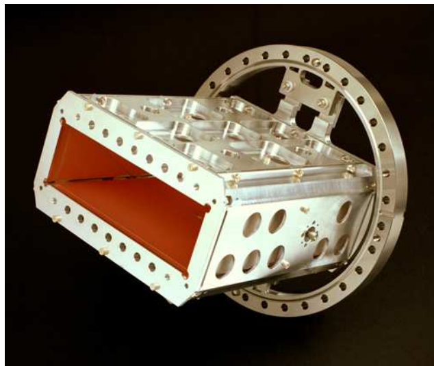
Figure 5.18: Linear cut position pick-up from the GSI synchrotron ring with an aperture limitation of 200 \times 70 \text{ mm}^2 .
