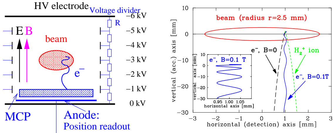
Figure 3.20: Left: Schematic trajectory of an electron in an ionization profile monitor in the presence of a homogeneous electric E and magnetic field B . Right: The comparison of the trajectories of an H_2^+ -ion and an electron with and without a magnetic field visualizes the broadening due to the beam space charge field. By applying a magnetic field the electron is fixed to the field line, as shown in the insert. The beam parameters are: 10^9 U^{73+} within a 10 m long bunch with radius 2.5 mm.
