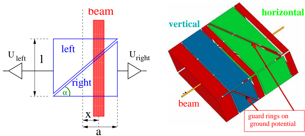
Figure 5.17: Left: Scheme of the position measurement using the so-called linear cut and an example of an electrode arrangement for the horizontal plane. Right: Schematic drawing for a linear cut BPM for both planes.
