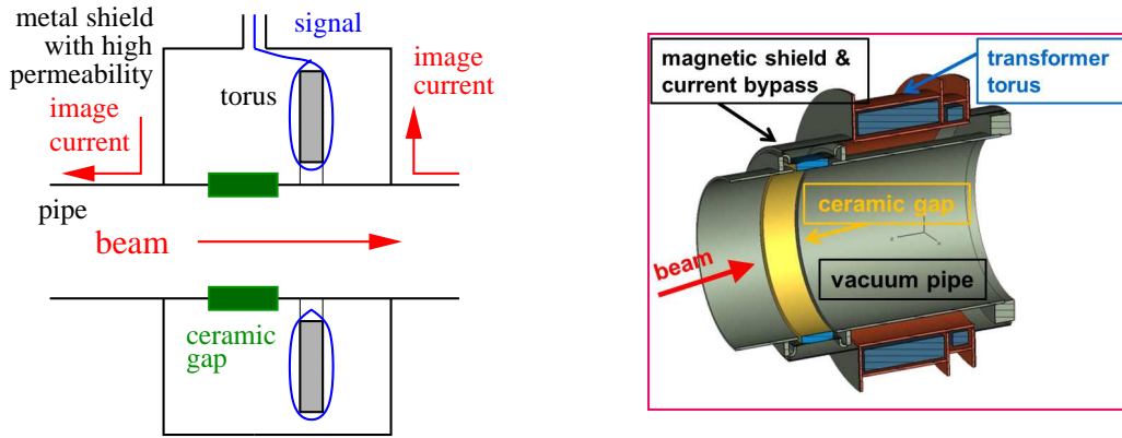
Figure 2.8: Left: The general scheme beam pipe intersected by a ceramic gap and a transformer housing as used as an image current pass and a shielding against external magnetic fields is shown. Right: The technical drawing for a transformer arrangement surrounding a beam pipe including the gap magnetical shield is shown.
