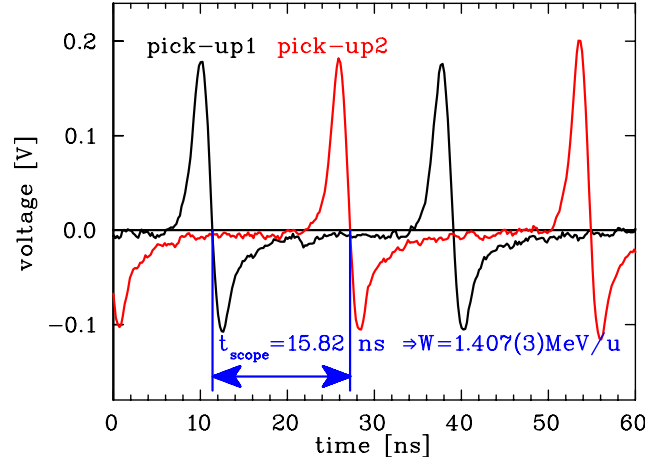
Figure 6.5: Time-of-flight signal from two pick-ups with W \simeq 1.4 MeV/u at the GSI-LINAC. The frequency is f_{rf} = 36.136 MHz \Leftrightarrow T = 1/f_{rf} = 27.673 ns. For the distance of L = 1.629 m between the pick-ups N = 3 bunches are between the pick-ups. Inserting the time difference of t_{scope} = 15.82 ns in Eq. 6.6, the velocity \beta = 0.05497(7) and the corresponding beam energy W = 1.407(3) MeV/u is calculated. The error is given by Eq. 6.7 inserting the uncertainties of \Delta t = 0.1 ns and \Delta L = 1 mm.
