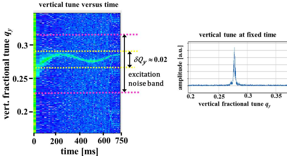
Figure 5.35: Left: Measurement of the tune at the GSI synchrotron for an \text{Ar}^{10+} beam accelerated from 11 to 300 MeV/u within 0.75 s [108]. Displayed is the Fourier transformation of displacements of successive individual bunches over 4096 turns excited by the depicted noise band during acceleration as a function of time. The maximum of the Fourier transformation is color-coded in a linear manner; \delta Q_y is the variation of the tune value. Right: Single tune spectrum 110 ms after the ramp start averaged over 4096 turns corresponding to \sim 15 ms.
