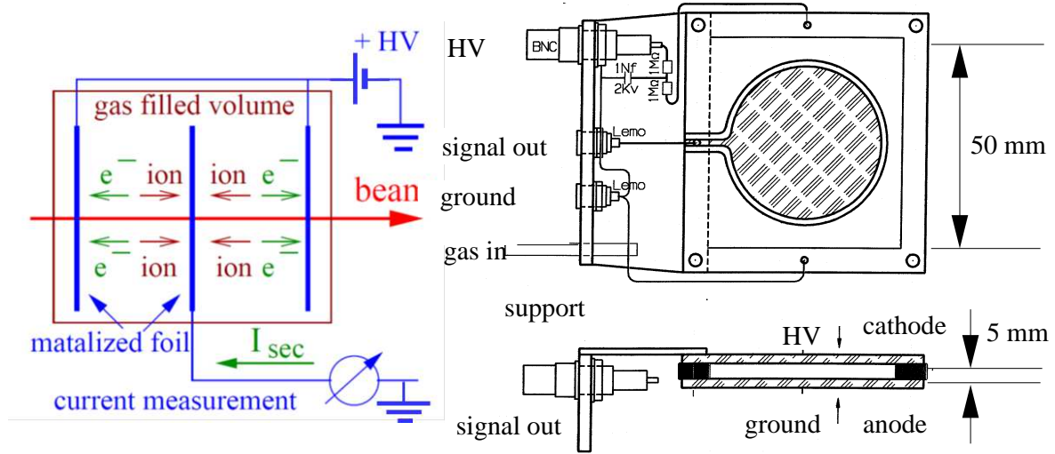
Figure 2.36: The scheme of an IC (left) and its realization with a 5 mm active length (right).
