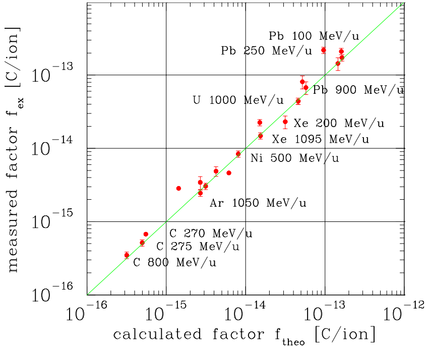
Figure 2.37: The measured calibration factor of an IC and calculated value using energy loss for various slowly extracted ion from the GSI synchrotron [17].
