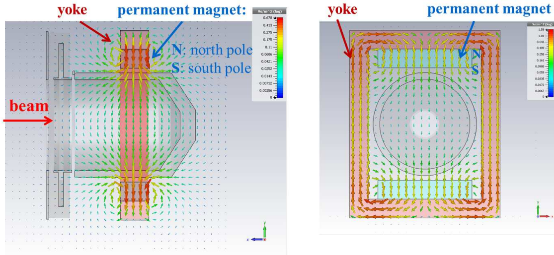
Figure 2.24: Magnetic field lines of the arrangement of Co-Sm permanent magnets within the yoke for the Faraday cup of Fig. 2.22. The homogeneous field strength is B \sim 0.06 T.
