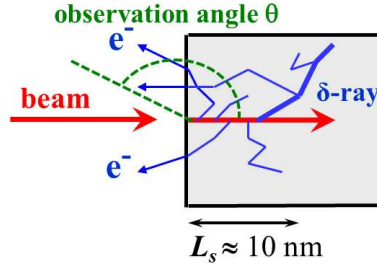
Figure 2.20: Schematic drawing of the secondary electron generation from a surface by charged particle impact; L_s is the scattering length from which electrons are able to reach the surface.
