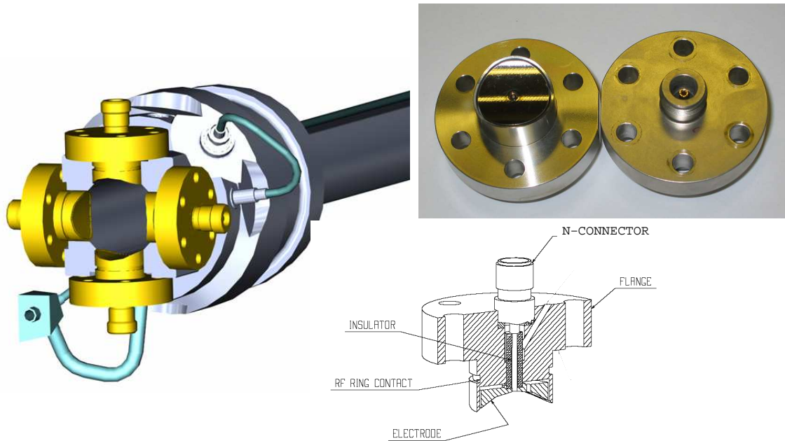
Figure 5.14: Left: The installation of the curved \text{\O} 24 mm button BPMs at the LHC beam pipe of \text{\O} 50 mm, from [86]. Right: Photo of a BPM used at LHC, the air side is equipped with a N-connector as well as a technical drawing for this type.
