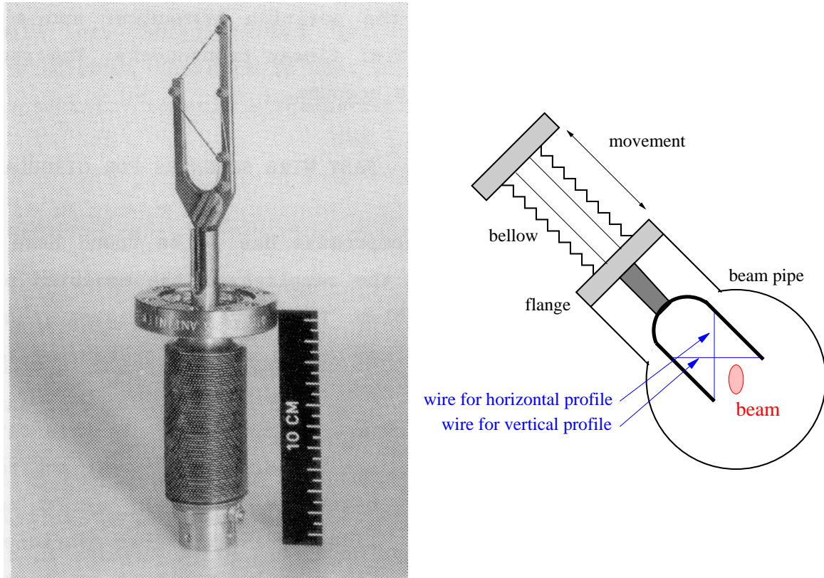
Figure 3.11: Linear scanner used at CERN [38].
