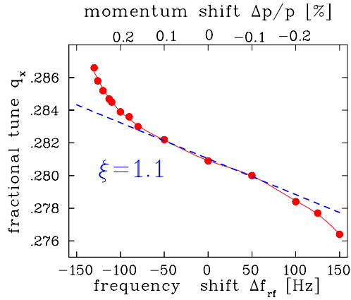
Figure 5.37: Measurement of the chromaticity at LEP. The horizontal tune is determined for different setting of the acceleration frequency and therefore of the momentum of the circulating beam. The chromaticity is fitted through the linear part of the data [110].
