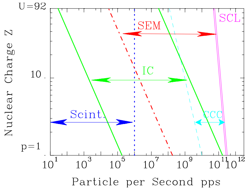
Figure 2.30: Overview of the different detector systems used for slow extraction at the GSI synchrotron. The numbers are given for the different ions with a kinetic energy of 1 GeV/u, extracted within 1 s and a spot size of 1 cm 2 . With a scintillator up to 10 6 particles can be counted. The lower limit of the IC and SEM correspond to a secondary current of 1 pA, the upper threshold of the IC is 30 Gray/s. The CCC (cryogenic current comparator) measures the magnetic field. SCL means the incoherent space-charge limit of the synchrotron at injection energy.
