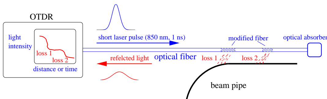
Figure 8.9: Principle of an OTDR beam loss detection with optical fibers.
