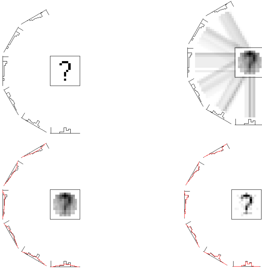
Figure 6.10: Schematic plots for the tomographic reconstruction technique [115]. The original 2 dimensional image and the 1-dim projections are shown to the left. A first back projection is shown top right. The first iteration step for the generation of the differences in the projected data is plotted bottom left. After \sim 50 iterations, the original image can be reconstructed.
