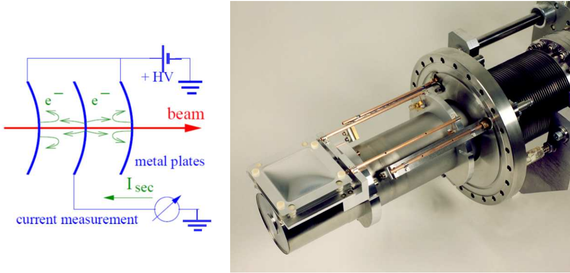
Figure 2.39: Scheme of a SEM (left) and a photo of the SEM part made of 3 Al foils with thickness of 100 \mu\text{m} of the feed-through used for slow extraction current measurements at GSI.
