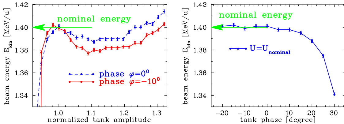
Figure 6.6: The output energy of the GSI-LINAC as a function of the applied rf-amplitude inside the tank (left) and phase for the nominal amplitude (right) as recorded like displayed in Fig. 6.5. The required energy of this module is 1.400 MeV/u. The distance between the pick-ups is in this case L = 1.97 m with N = 4 bunches between.
