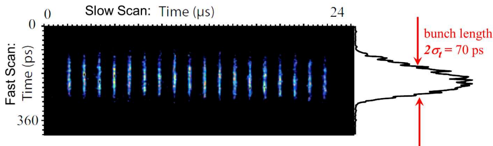
Figure 6.26: Bunch length measurement with a streak camera, using synchrotron light from individual bunches emitted by the passage through a dipole at SOLEIL [127]. The horizontal axis scaling is 24 \mu\text{s} full scale for the bunch repetition (slow scan direction) and the vertical axis is 360 \text{ ps} full scale for the bunch structure (fast scan direction). The bunch width is \sigma \simeq 35 \text{ ps} as achieved for a medium current of 12 \text{ mA} and a rf-voltage of 2 \text{ MV} , see Fig. 6.27 for a compilation of such measurements.
