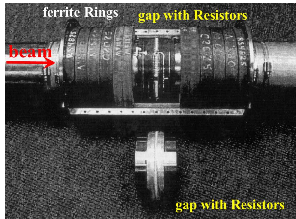
Figure 6.14: Photo of the wall current monitor used at FERMI-Lab for protons, from [117]. The ceramic gap is shown separately. The ferrite rings and the printed circuit with the resistors are visible.
