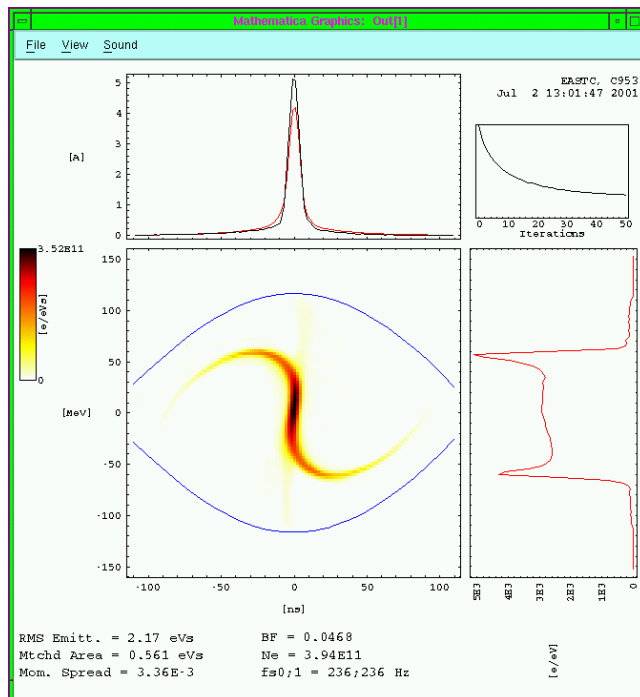
Figure 6.12: Same as Fig. 6.11 but for a mismatched bunch. The complex rotation of the bunch width is seen left and the reconstructed phase space density (right) for one specific time slice. The filamented distribution rotates to yield varying bunch shapes. Form [116].
