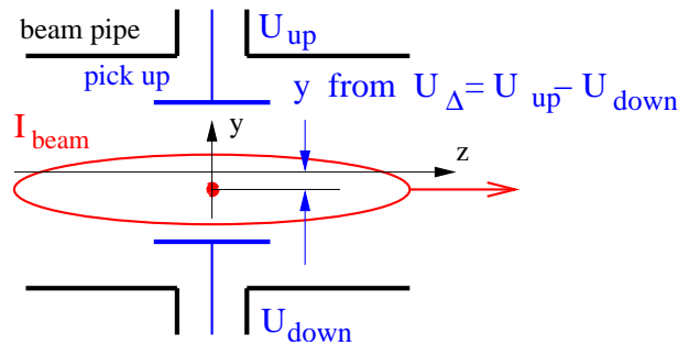
Figure 5.9: Schematics of a BPM for the vertical position reading based on the proximity effect.
