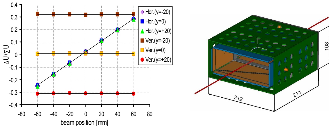
Figure 5.19: Left: Numerical calculation of the position reading \Delta U/\Sigma U as a function of beam displacement for the horizontal plane. The the simulated beam is swept in horizontal direction (curves with constant slope) and vertical direction (constant functions) and proves the decoupling of both planes [91]. Right The BPM geometry for these calculations is depicted right having a horizontal half-aperture of a = 100 mm and vertical half-aperture of b = 35 mm and a length of 211 mm comparable, to the one shown in Fig 5.18.
